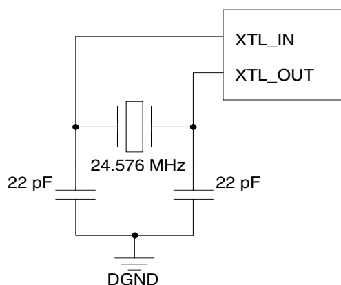
Figure 17. External Crystal
