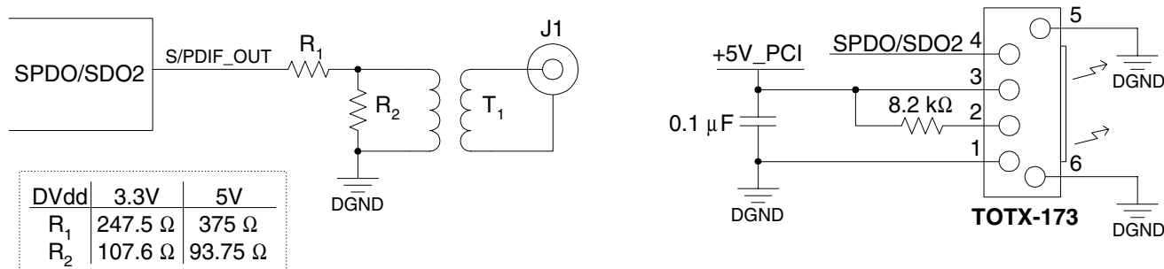
Figure 15. S/PDIF Output
