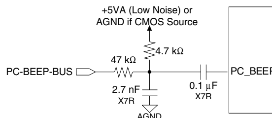
Figure 22. PC_BEEP Input
