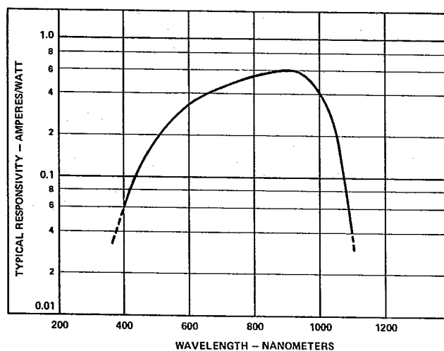
Figure 2 — Typical Spectral Responsivity Characteristic
