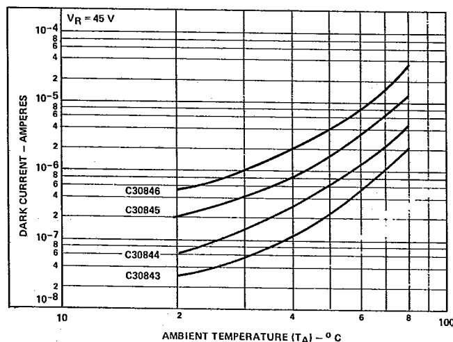
Figure 3 — Typical Dark Current vs Ambient Temperature
