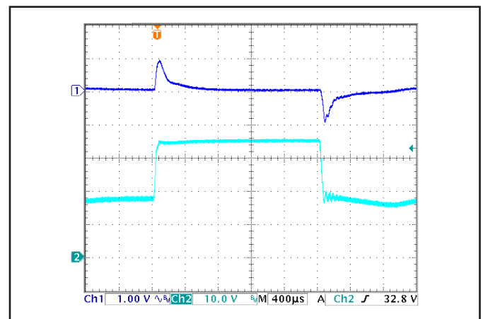
Figure 6: Output voltage response to step-change in input voltage (500 V/ms). Load cap: 100 \mu\text{F} , electrolytic output capacitance. Ch 1: V out (1 V/div), Ch 2: V in (10 V/div).
