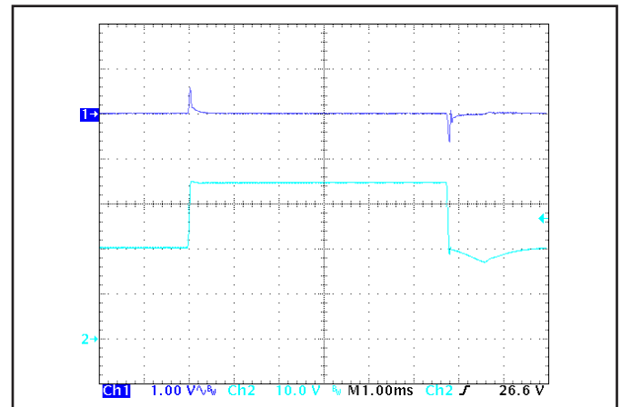
Figure 6: Output voltage response to step-change in input voltage (1000 V/ms). Load cap: 100 \mu F , electrolytic output capacitance. Ch 1: Vout (1 V/div), Ch 2: Vin (10 V/div).
