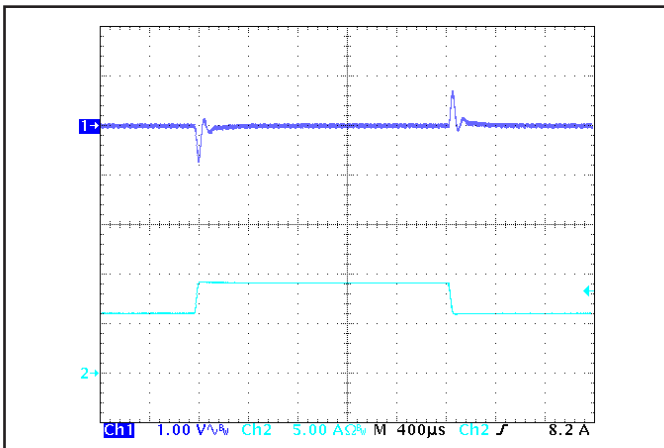
Figure 5: Output voltage response to step-change in load current (50%-75%-50% of I_{out(max)} ); dI/dt = 0.1 A/\mu s . Load cap: 1 \mu F ceramic capacitor. Ch 1: Vout (1 V/div), Ch 2: Iout (5 A/div).
