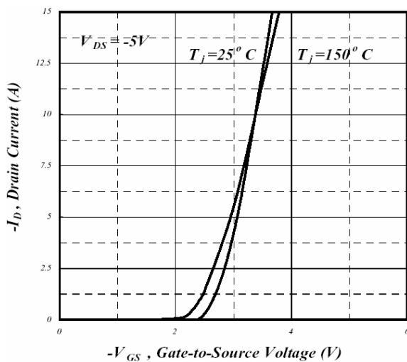
Fig 11. Transfer Characteristics
