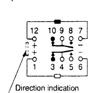
Schematic (Top view)
