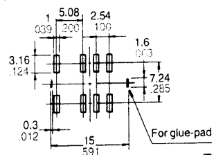
Schematic (Top view)
