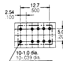
PC board pattern (Copper side view)
