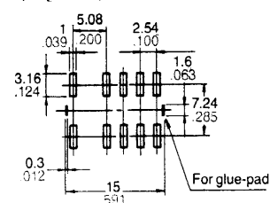
Suggested mounting pad (Top view)
