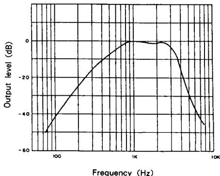
C-message filter frequency characteristics
