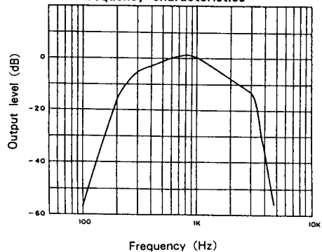
Audio measurement circuit frequency characteristics
