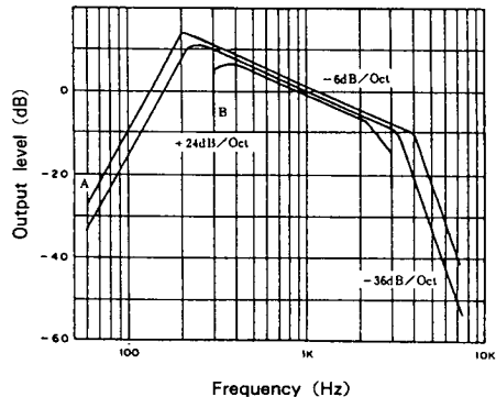
Audio measurement circuit frequency characteristics
