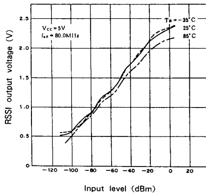
RSSI characteristics (MIX IN/RSSI OUT)
