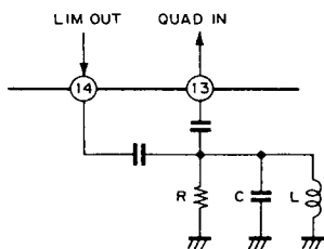
RLC phase shifter
