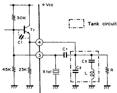
Colpitts type crystal oscillation circuit
