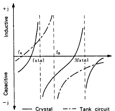
Reactance characteristics
