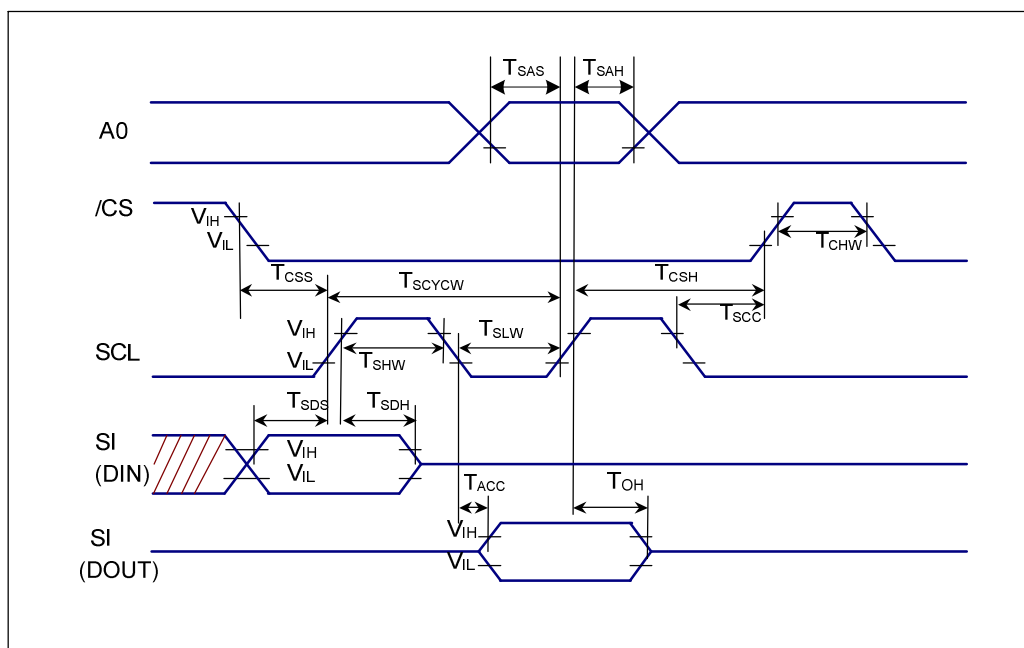
Figure 11.4-1 4-pin Serial Interface Characteristics
