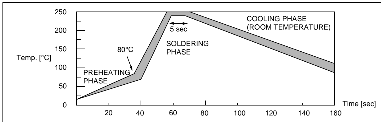
Figure 119. Recommended Reflow Soldering Oven Profile (MID JEDEC)
