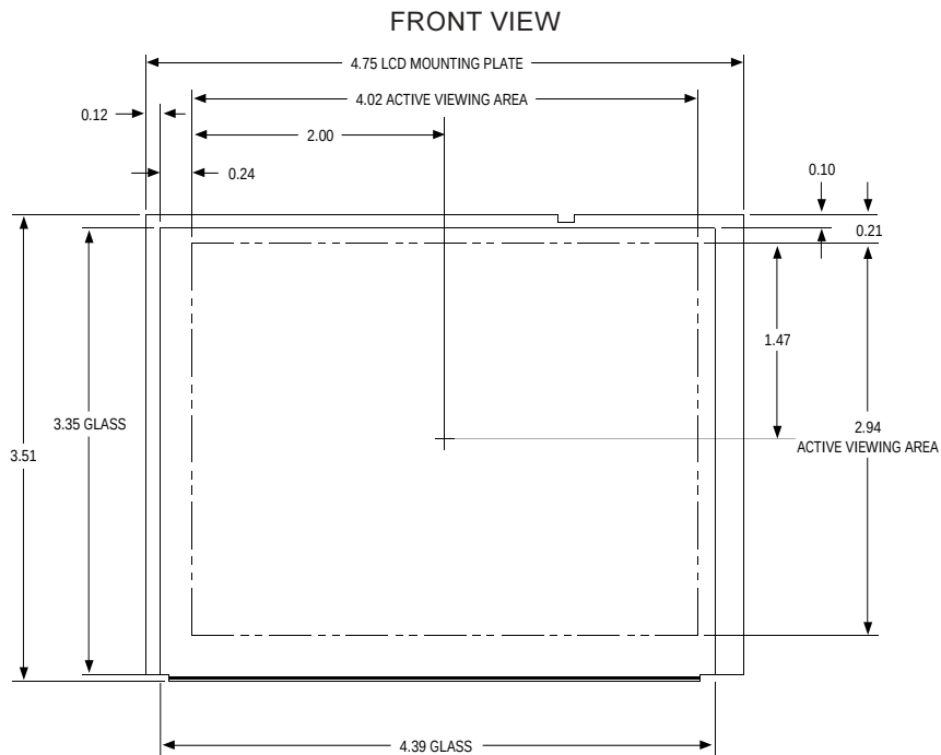
FIG. 2 MECHANICAL OUTLINE DIMENSIONS
