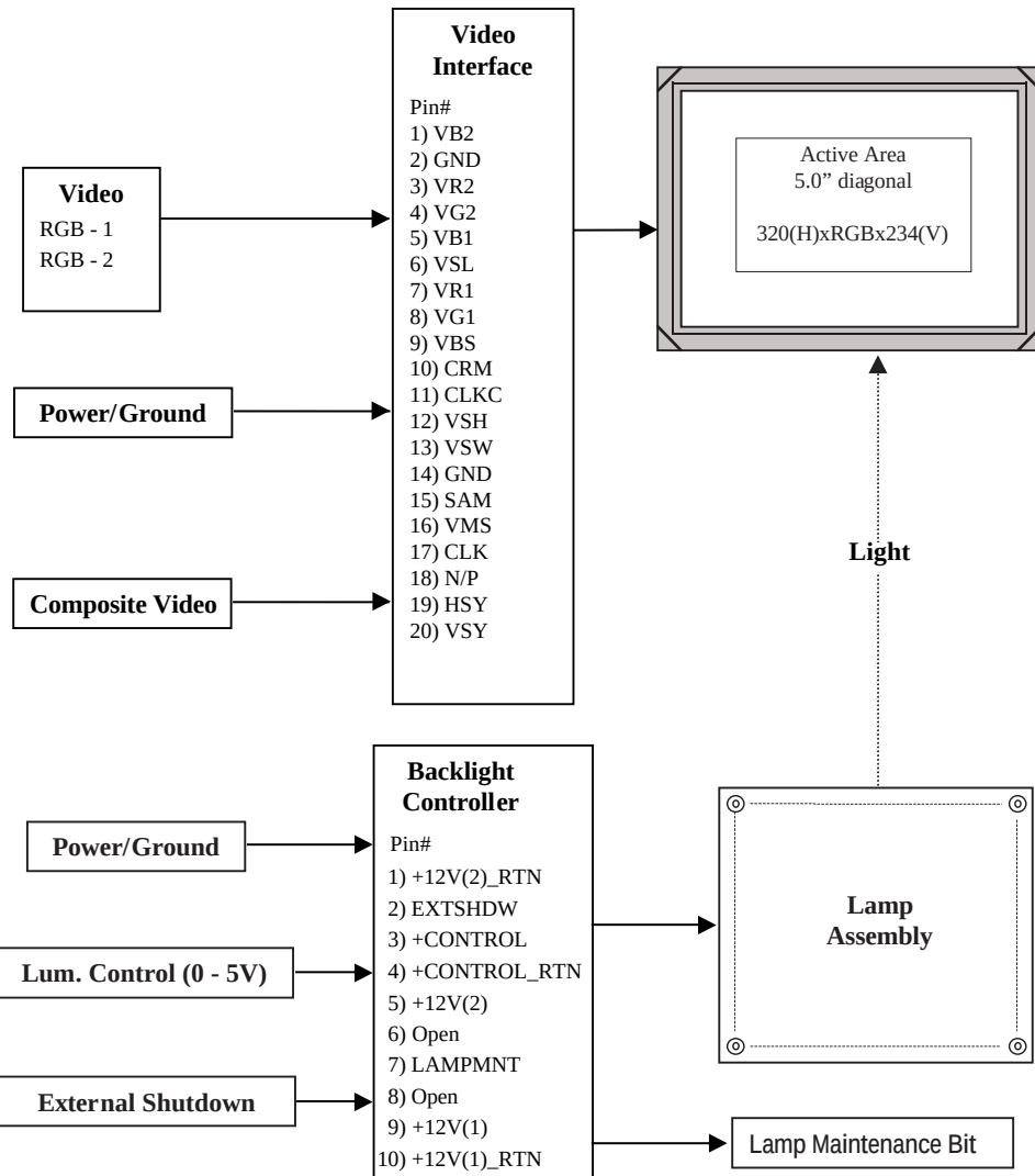
FIG. 1 DISPLAY HEAD ASSEMBLY BLOCK DIAGRAM
