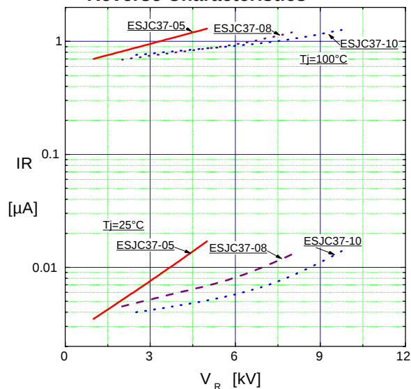
Reverse Characteristics
