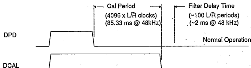
Figure 6. Initial Calibration Cycle Timing
