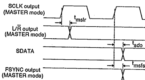
SCLK to SDATA, L/R &amp; FSYNC - MASTER Mode
