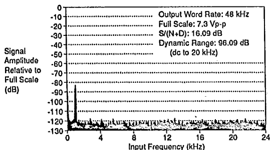
Figure 9. CS5336 FFT Plot with -80 dB, 1 kHz Input
