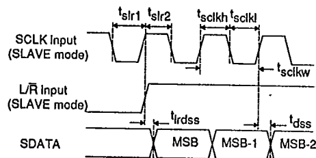
SCLK to L/R &amp; SDATA - SLAVE mode, FSYNC high
