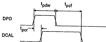
Power Down &amp; Calibration Timing
