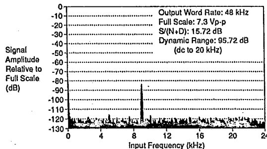
Figure 10. CS5336 FFT Plot with -80 dB, 9 kHz Input
