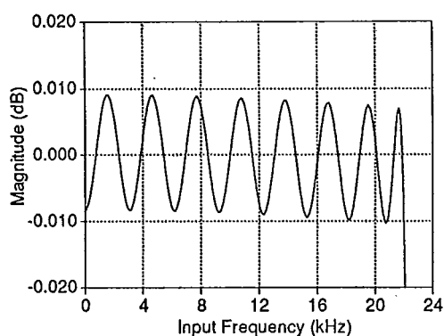
Figure 14. CS5338/9 Digital Filter Passband Ripple
