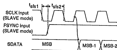
FSYNC to SCLK - SLAVE Mode, FSYNC Controlled.
