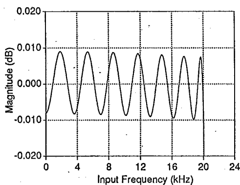
Figure 15. CS5336/7 Digital Filter Passband Ripple
