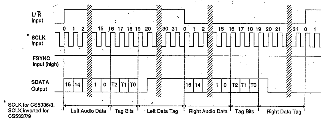
Figure 4. Data Output Timing - SLAVE Mode, FSYNC high
