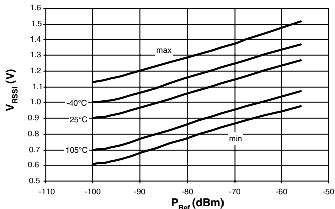
Figure 8. RSSI Characteristic
