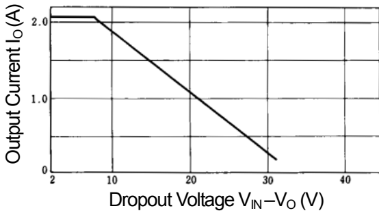
NJM7800 Series Short Circuit Output Current ( T_j=25^\circ\text{C} , \infty Heat Sink)
