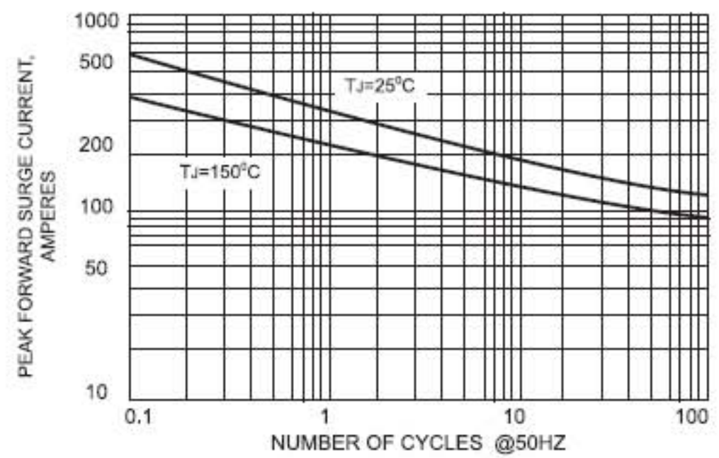
FIG.2 - NON-REPETITIVE PEAK FORWARD SURGE CURRENT
