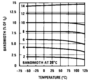
Typical Bandwidth Variation
