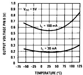
Typical Output Voltage vs Temperature
