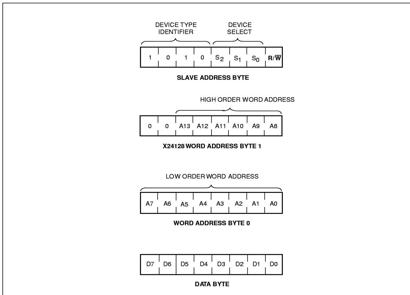
Figure 4. Device Addressing
