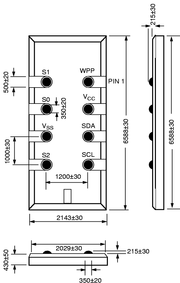
X24128: Bottom View
