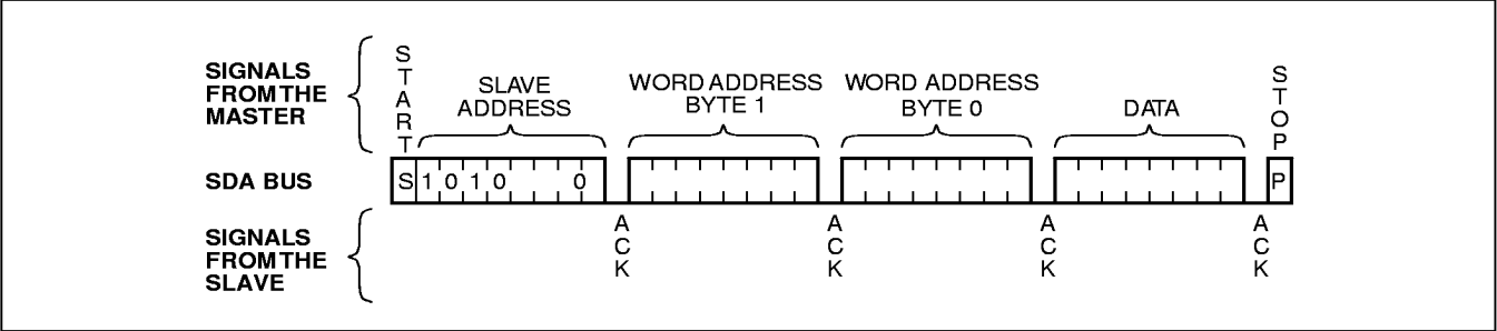
Figure 5. Byte Write Sequence
