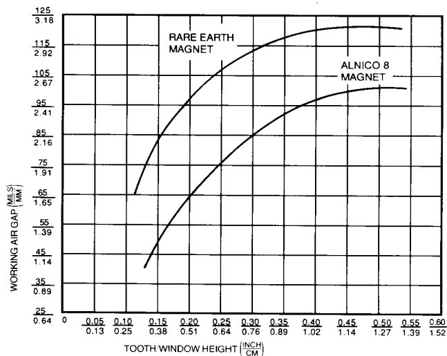
WORKING AIR GAP vs TOOTH WINDOW HEIGHT FIGURE 5
