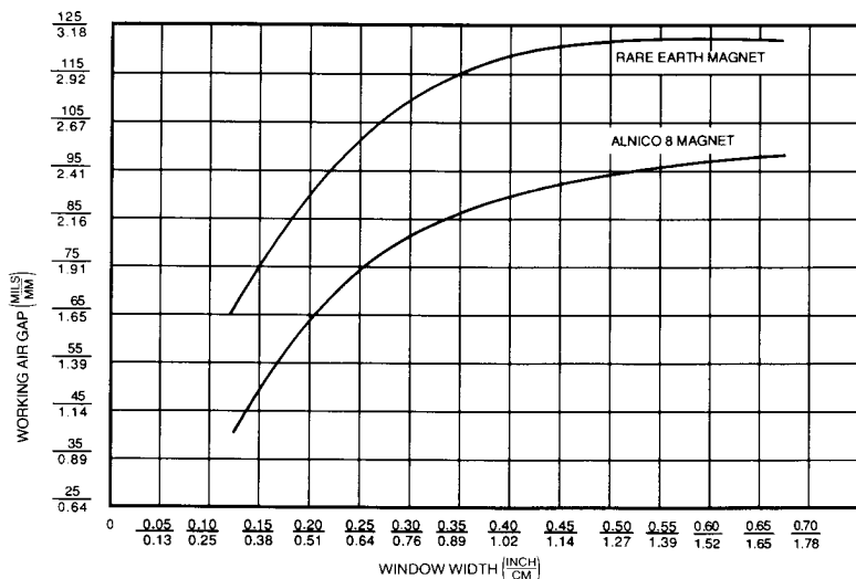
WORKING AIR GAP vs WINDOW WIDTH at +25°C FIGURE 6
