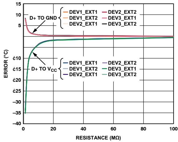
Figure 8. Remote Temperature Error vs. PCB Resistance
