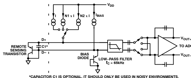
Figure 14. Signal Conditioning for Remote Diode Temperature Sensors
