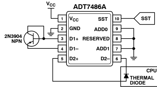
Figure 18. ADT7486A Typical Application Schematic
