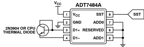
Figure 17. ADT7484A Typical Application Schematic
