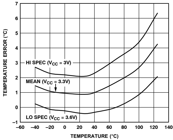
Figure 4. Local Temperature Error
