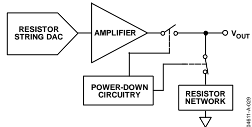
Figure 28. Output Stage During Power-Down
