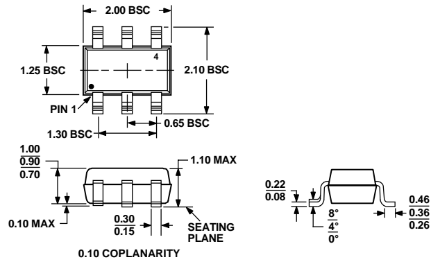
Figure 37. 6-Lead Plastic Surface Mount Package [SC70] (KS-6)
