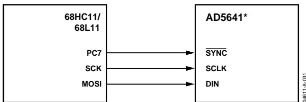
Figure 30. AD5641 to 68HC11/68L11 Interface
