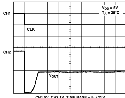
Figure 20. Exiting Power-Down
