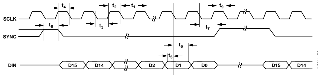
Figure 2. Timing Diagram
