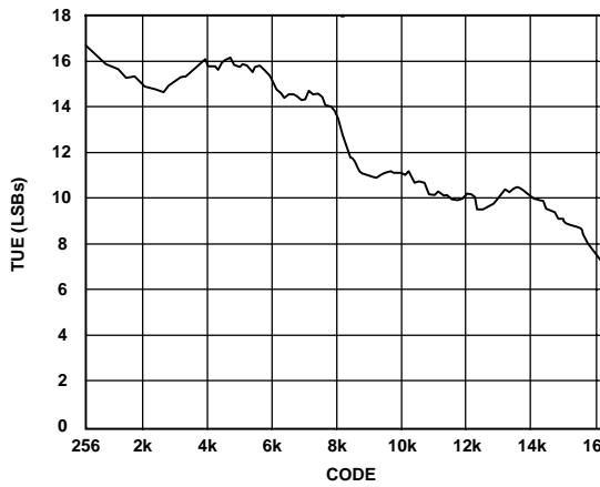
Figure 5. Total Unadjusted Error
