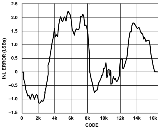
Figure 4. Typical INL Plot
