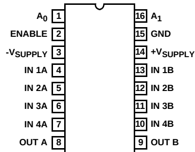
HI-549 (CERDIP, PDIP, SOIC)
