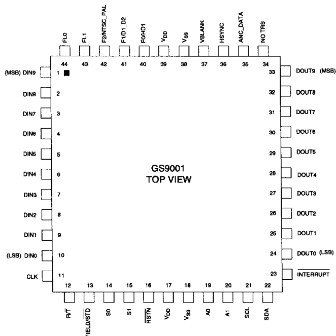
Fig. 1 GS9001 EDH Coprocessor Pin Connections
