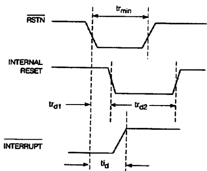
Fig. 2b Reset and Interrupt Timing
