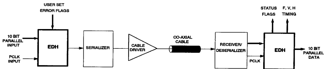
Fig. 8 GS9001 System Placement
