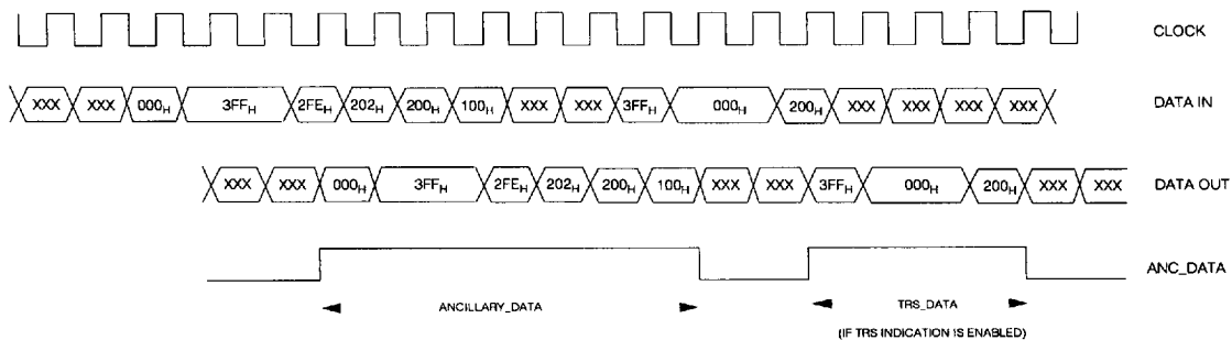
Fig. 4 Ancillary Data Indication Timing
