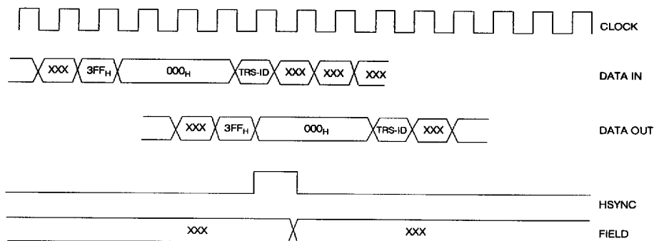
Fig. 6 Composite Timing Signals
