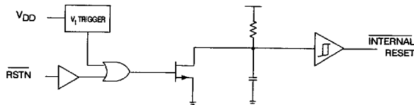
Fig. 2a GS9001 Internal Reset Circuit
