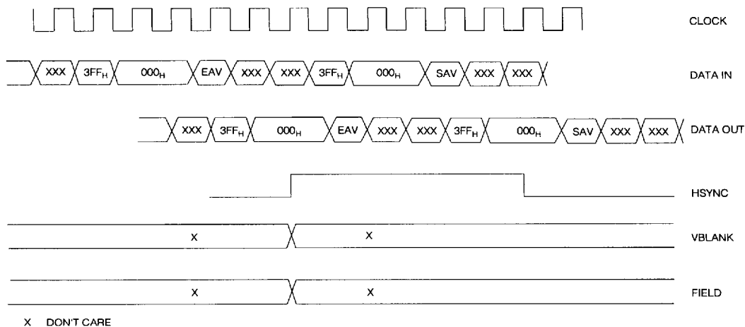
Fig. 5 Component Timing Signals
