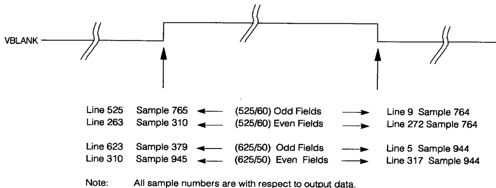
Fig. 6 Composite Timing Signals
