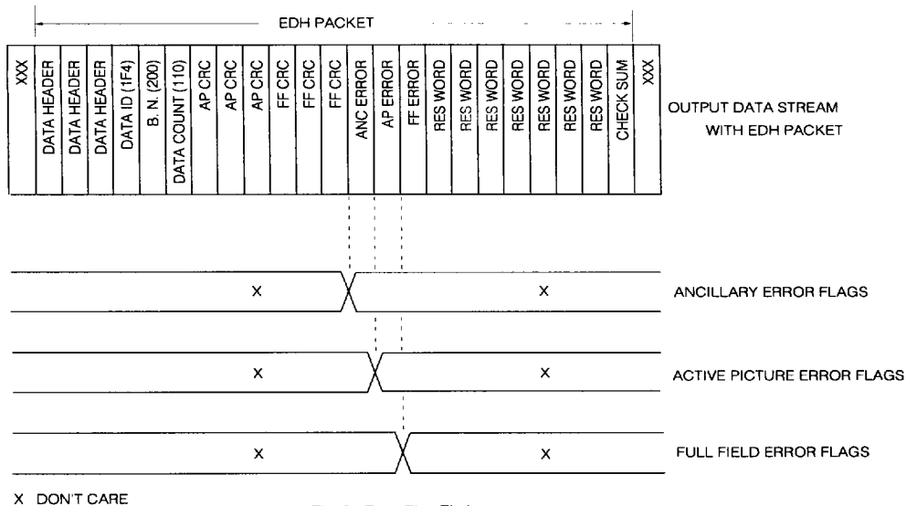
Fig. 3 Error Flag Timing
