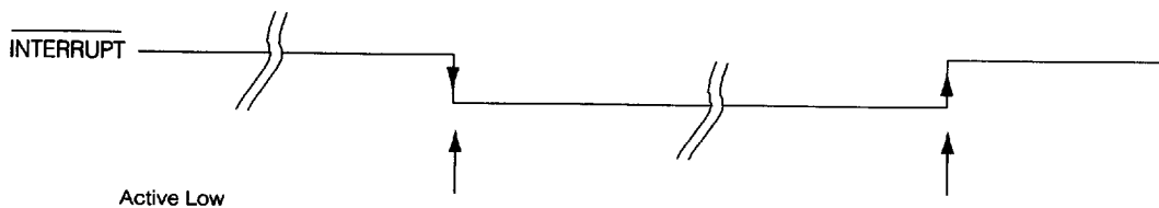
Fig. 2b Reset and Interrupt Timing
