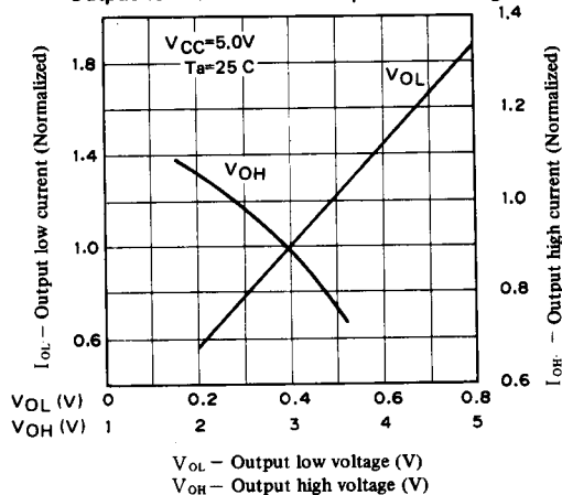
Output high current vs. Output high voltage Output low current vs. Output low voltage
