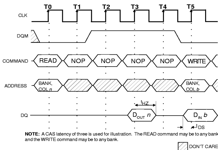
Figure 10 READ TO WRITE WITH EXTRA CLOCK CYCLE
