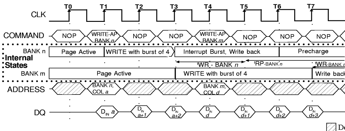
Figure 27 WRITE WITH AUTO PRECHARGE INTERRUPTED BY A WRITE
