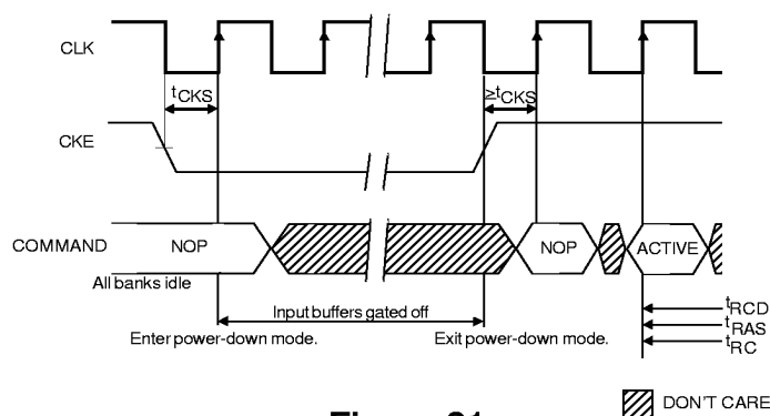
Figure 21 POWER-DOWN
