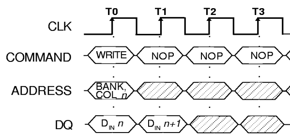
Figure 14 WRITE BURST
