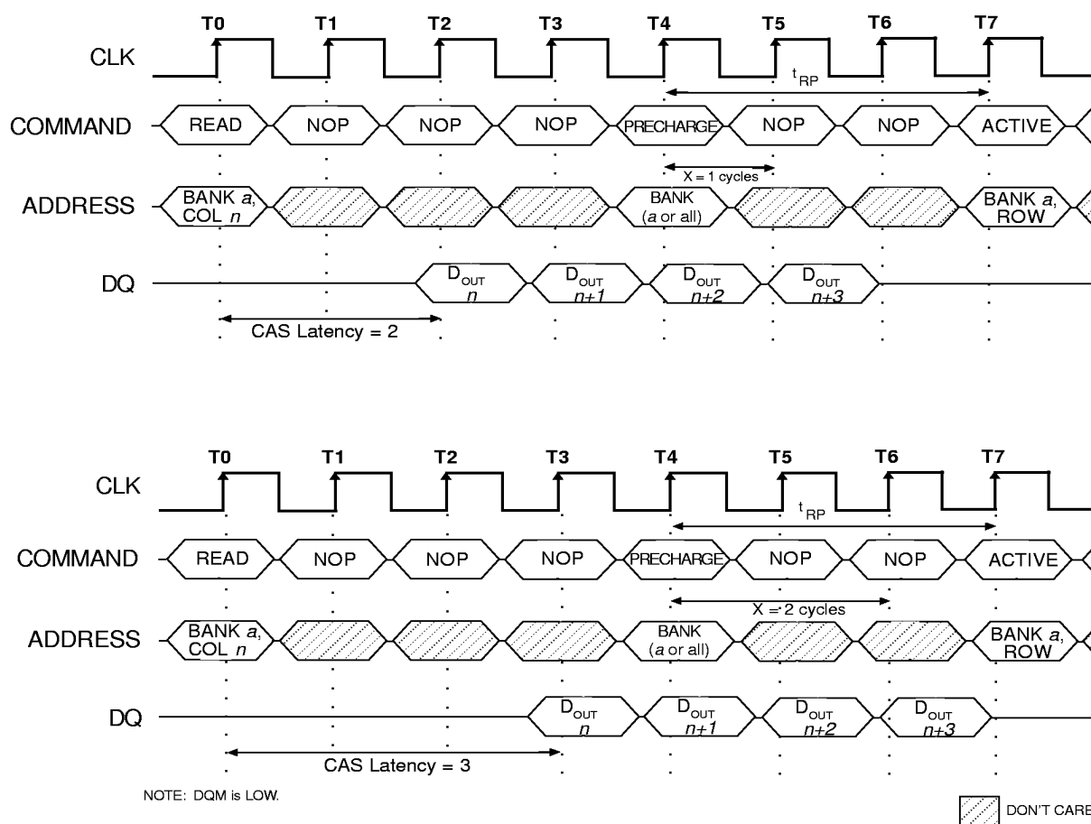
Figure 11 READ TO PRECHARGE
