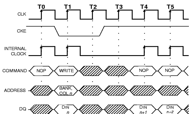
Figure 22 CLOCK SUSPEND DURING WRITE BURST
