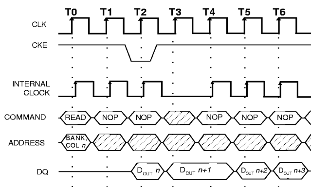
Figure 23 CLOCK SUSPEND DURING READ BURST
