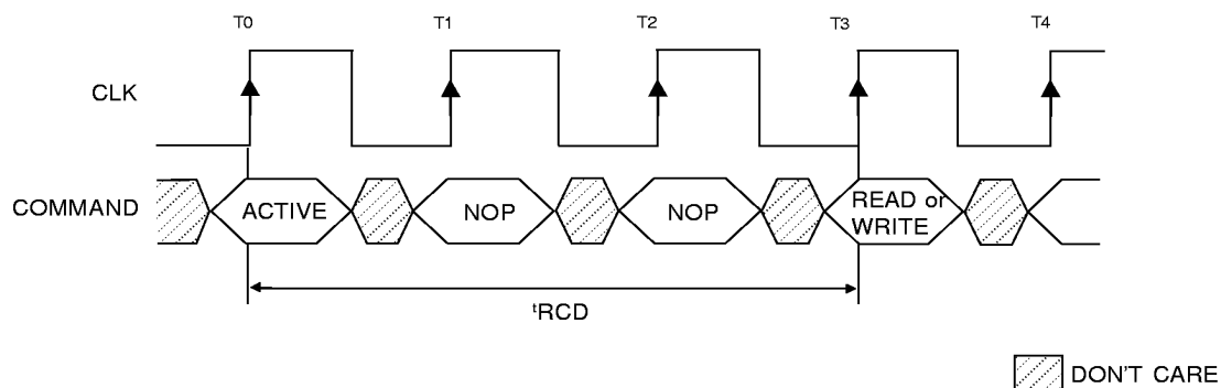
Figure 4 EXAMPLE: MEETING t_{RCD}(\text{MIN}) WHEN 2 < t_{RCD}(\text{MIN})/t_{CK} \leq 3
