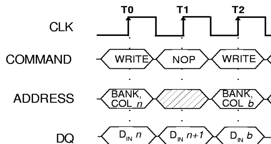
Figure 14 WRITE BURST
