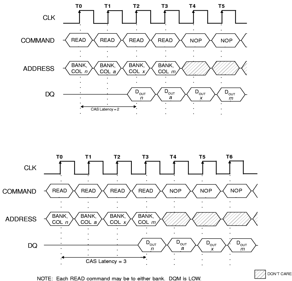
Figure 8 RANDOM READ ACCESSES
