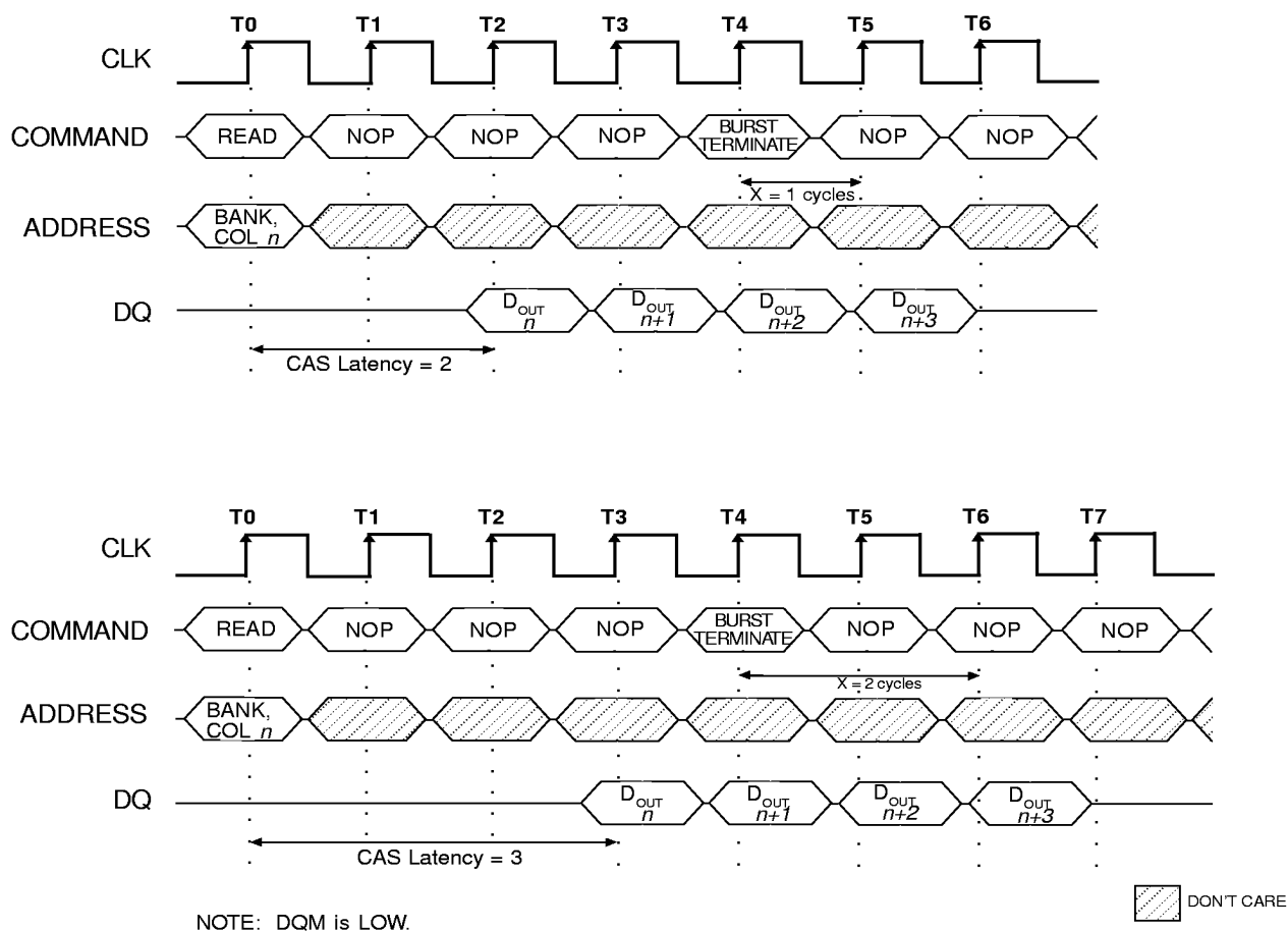
Figure 12 TERMINATING A READ BURST
