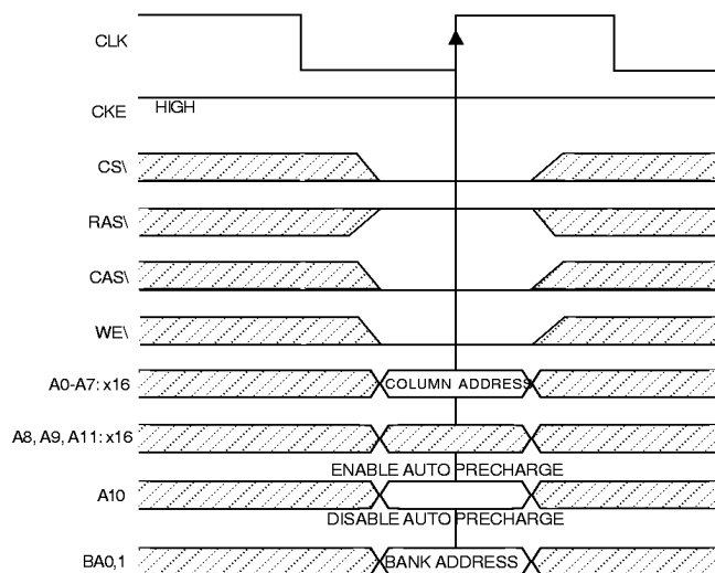
Figure 13 WRITE COMMAND
