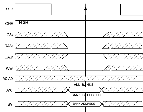
Figure 20 PRECHARGE COMMAND
