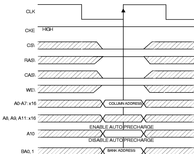
Figure 5 READ COMMAND
