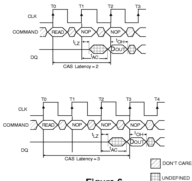
Figure 6 CAS LATENCY
