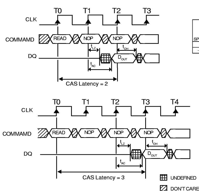
Figure 2 CAS LATENCY
