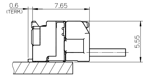
嵌合図 MATED CONNECTORS
