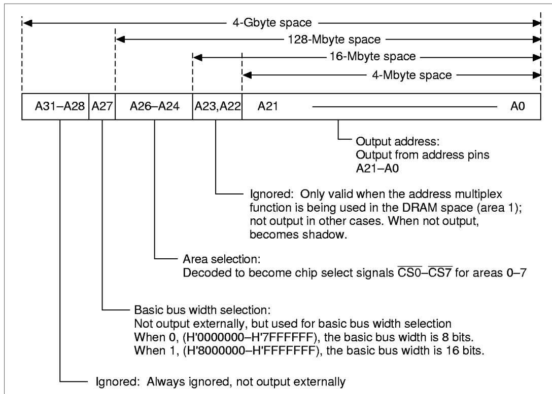
Figure 8.3 Address Format
