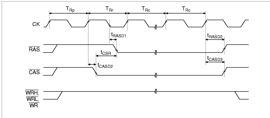
Figure 20.30 CAS-before-RAS Refresh (Long-Pitch)
