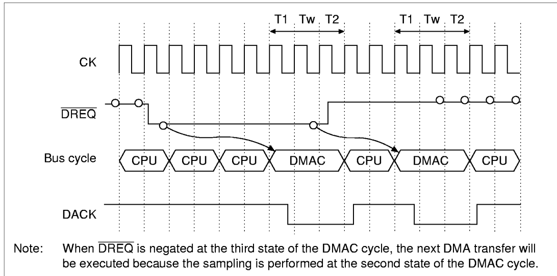
Figure 9.17 \overline{\text{DREQ}} Sampling Timing in Cycle-Steal Mode (Output with \overline{\text{DREQ}} Level Detection and DACK Active-Low) (Single Address Mode, Bus Cycle = 2 States + 1 Wait State)
