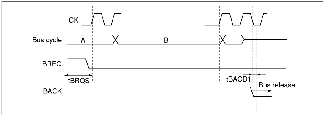
Figure 8.43 When \overline{\text{BREQ}} is Input without Satisfying \text{tBRQS}
