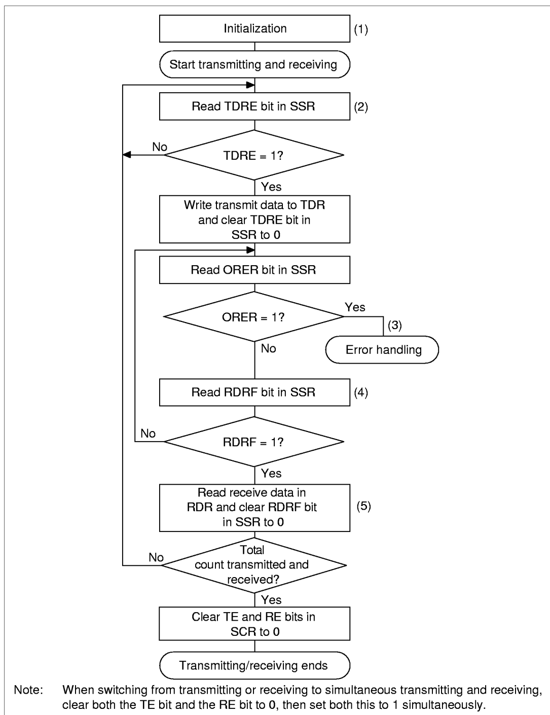
Figure 13.20 Sample Flowchart for Serial Transmitting and Receiving
