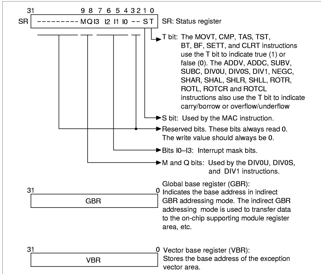
Figure 2.2 Control Registers
