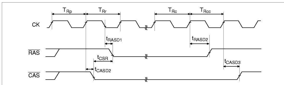
Figure 20.31 Self-Refresh
