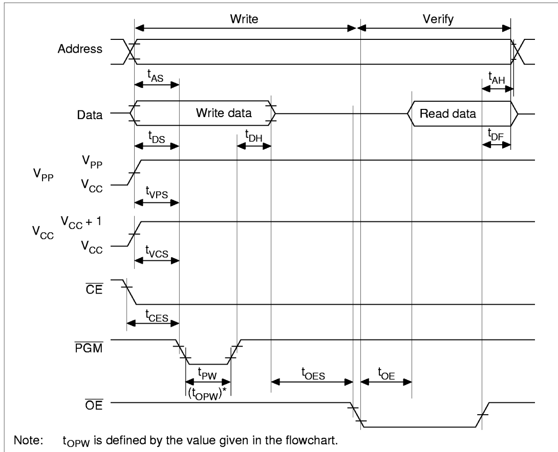
Figure 17.5 Write/Verify Timing
