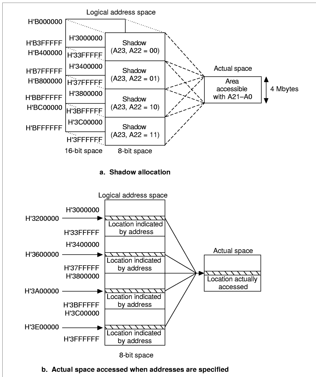
Figure 8.4 Shadows
