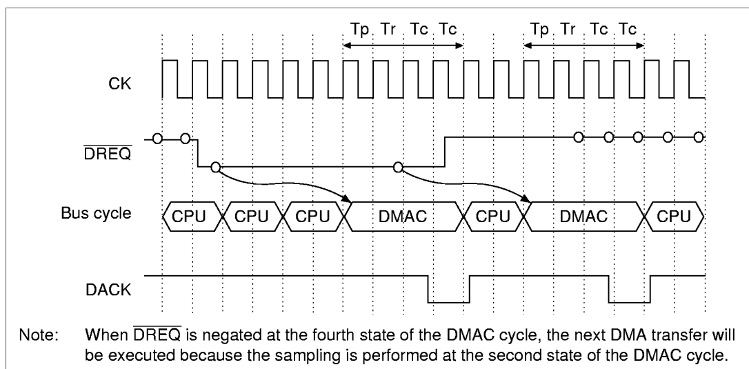
Figure 9.19 \overline{\text{DREQ}} Sampling Timing in Cycle-Steal Mode (Output with \overline{\text{DREQ}} Level Detection and DACK Active-Low) (Single Address Mode, Bus Cycle = DRAM Bus Cycle (Long Pitch Normal Mode))
