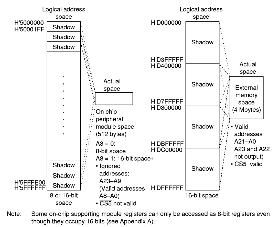
Figure 8.8 Memory Map of Area 5
