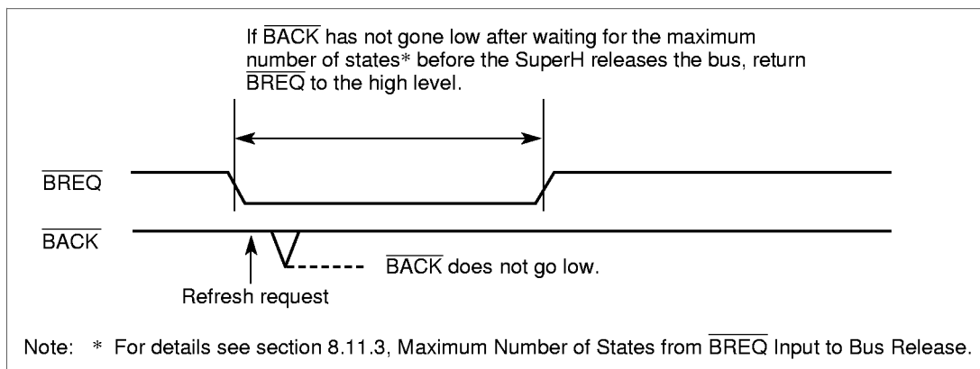
Figure 8.37 \overline{BACK} Operation in Response to Refresh Request (2)
