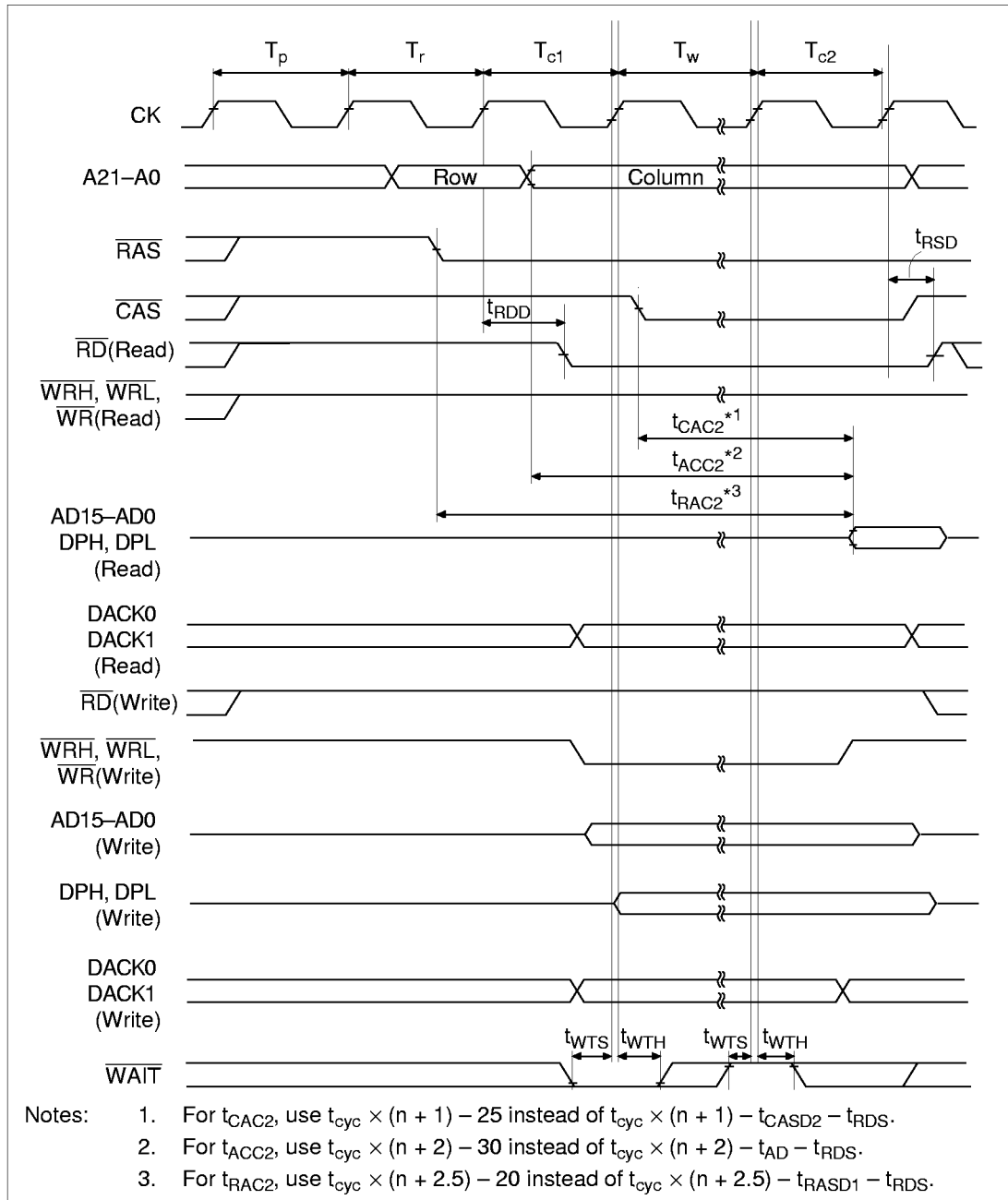
Figure 20.15 DRAM Bus Cycle: (Long-Pitch, High-Speed Page Mode + Wait State)
