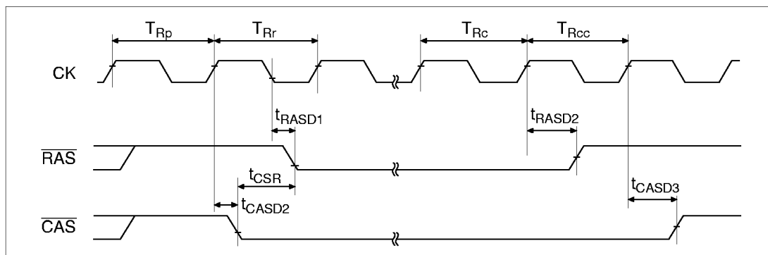
Figure 20.18 Self-Refresh
