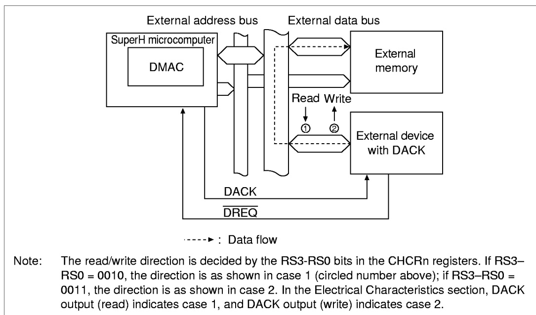
Figure 9.6 Data Flow in Single Address Mode
