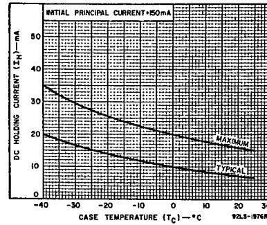
Fig. 10—DC holding current (positive or negative) vs. case temperature for T2302 series.
