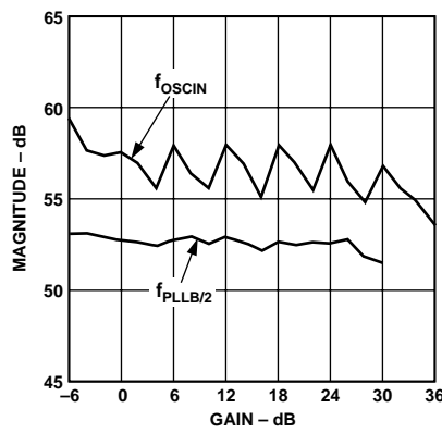
TPC 40. Rx Path SNR vs. Gain
