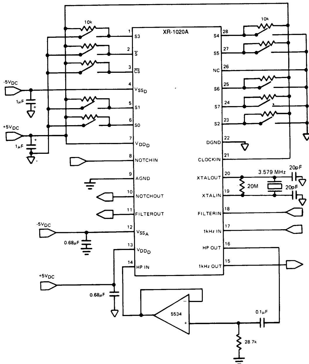
Figure 2. Typical Test Circuit
