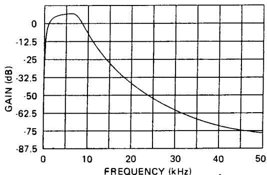
Figure 15. Amplitude Response: Program Weighting Filter
