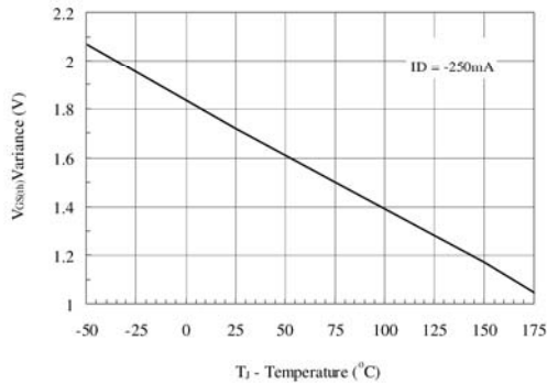
Threshold Voltage
