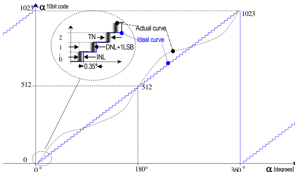
Figure 24: Integral and differential Non-Linearity (example)
