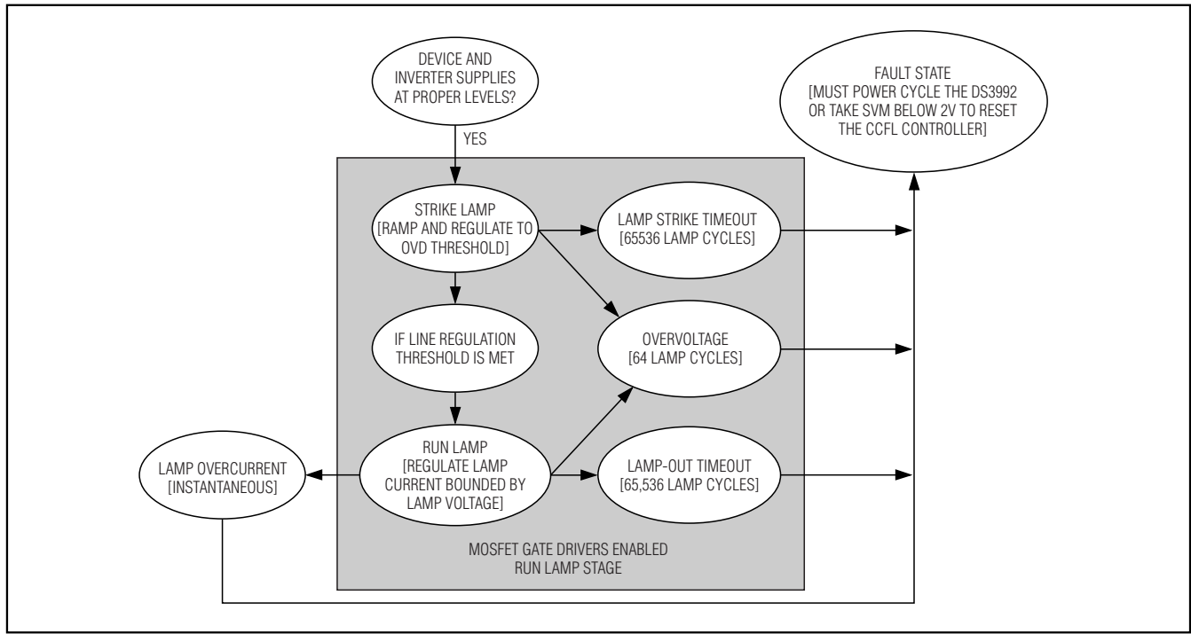
Figure 4. Fault-Handling Flowchart
