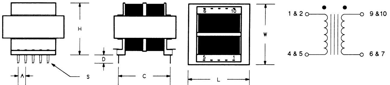
Dimensions, Inches
