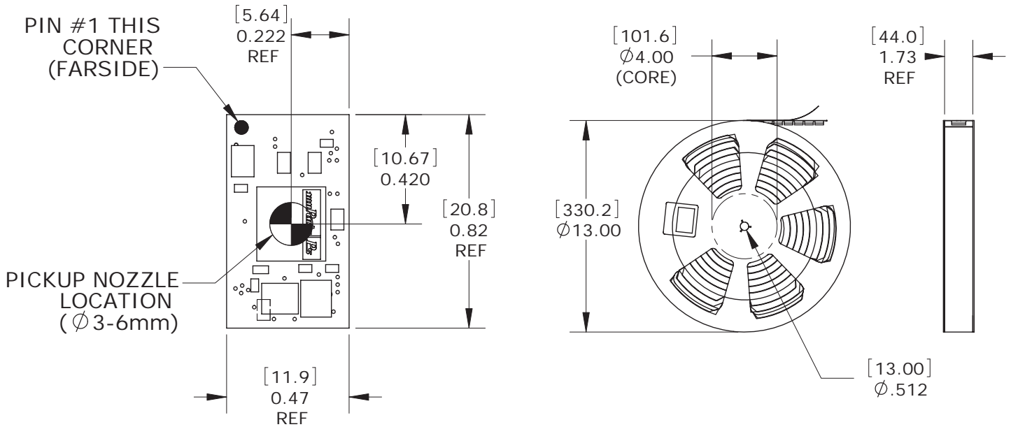
REEL INFORMATION (400 UNITS PER REEL)
