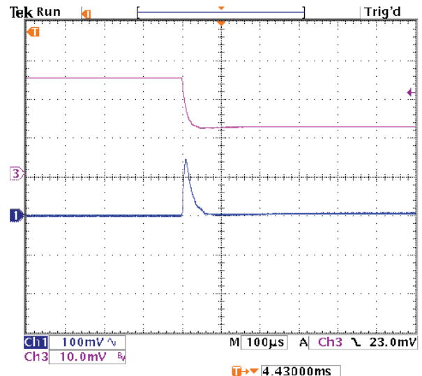
Step Load Transient Response (Vin=12V, Vout=5V, Clod=0, Iout=5A to 2.5A) Trace 1=Vout, 100 mV/div. Trace 3=Iout, 2A/div.
