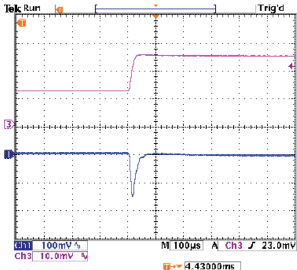
Step Load Transient Response (Vin=12V, Vout=5V, Clod=0, Iout=2.5A to 5A) Trace 1=Vout, 100 mV/div. Trace 3=Iout, 2A/div.
