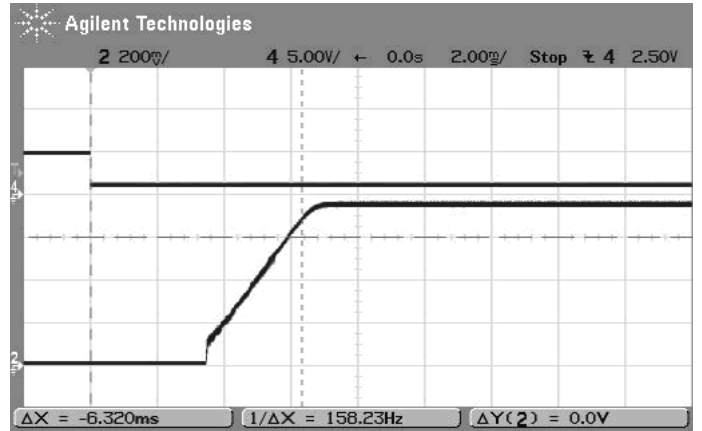
On/Off Enable Startup Delay (VIN=12V, Vout=0.75V, Iout=3A, Cload=0) Trace 4=Enable In, Trace2=Vout
