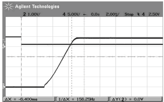
On/Off Enable Startup Delay (Vin=12V, Vout=5V, Iout=5A, Clod=0 Trace 4=Enable In, Trace2=Vout)
