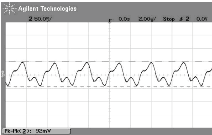
Output Ripple and Noise (Vin=12V, Vout=5V, Iout=5A, Clod=0, ScopeBW=100MHz)
