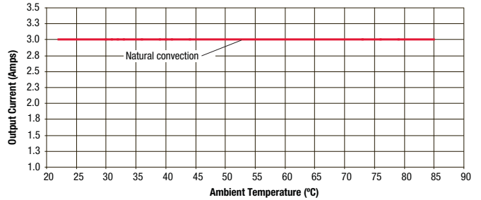
OKY-T/3-D12 Maximum Current Temperature Derating @ Sea Level (VIN = 12V, VOUT = 1.2V, airflow is transverse)
