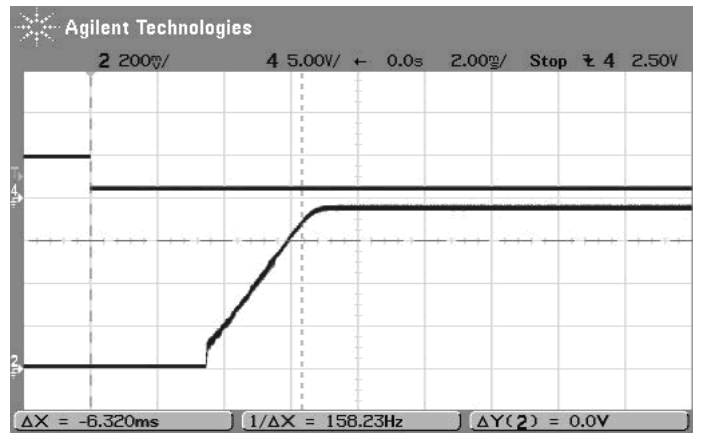
On/Off Enable Startup Delay (Vin=12V, Vout=0.75V, Iout=5A, Cload=0) Trace 4=Enable In, Trace2=Vout
