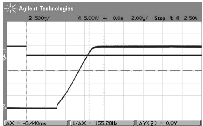
On/Off Enable Startup Delay (Vin=12V, Vout=2.5V, Iout=5A, Cload=0) Trace 4=Enable In, Trace 2=Vout
