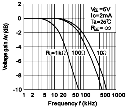
Fig.11 Frequency Response
