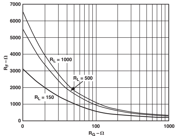
Figure 6b. Feedback Resistor Selection
