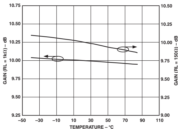
TPC 3. Gain vs. Temperature at 100\text{ MHz} ( A_V = 10\text{ dB} )
