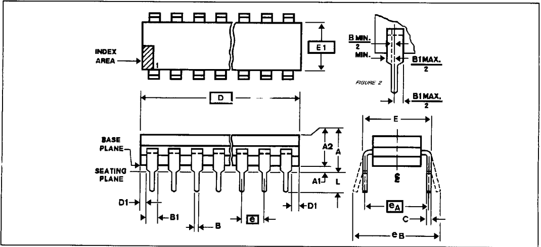
28 PINS CERDIP .300
