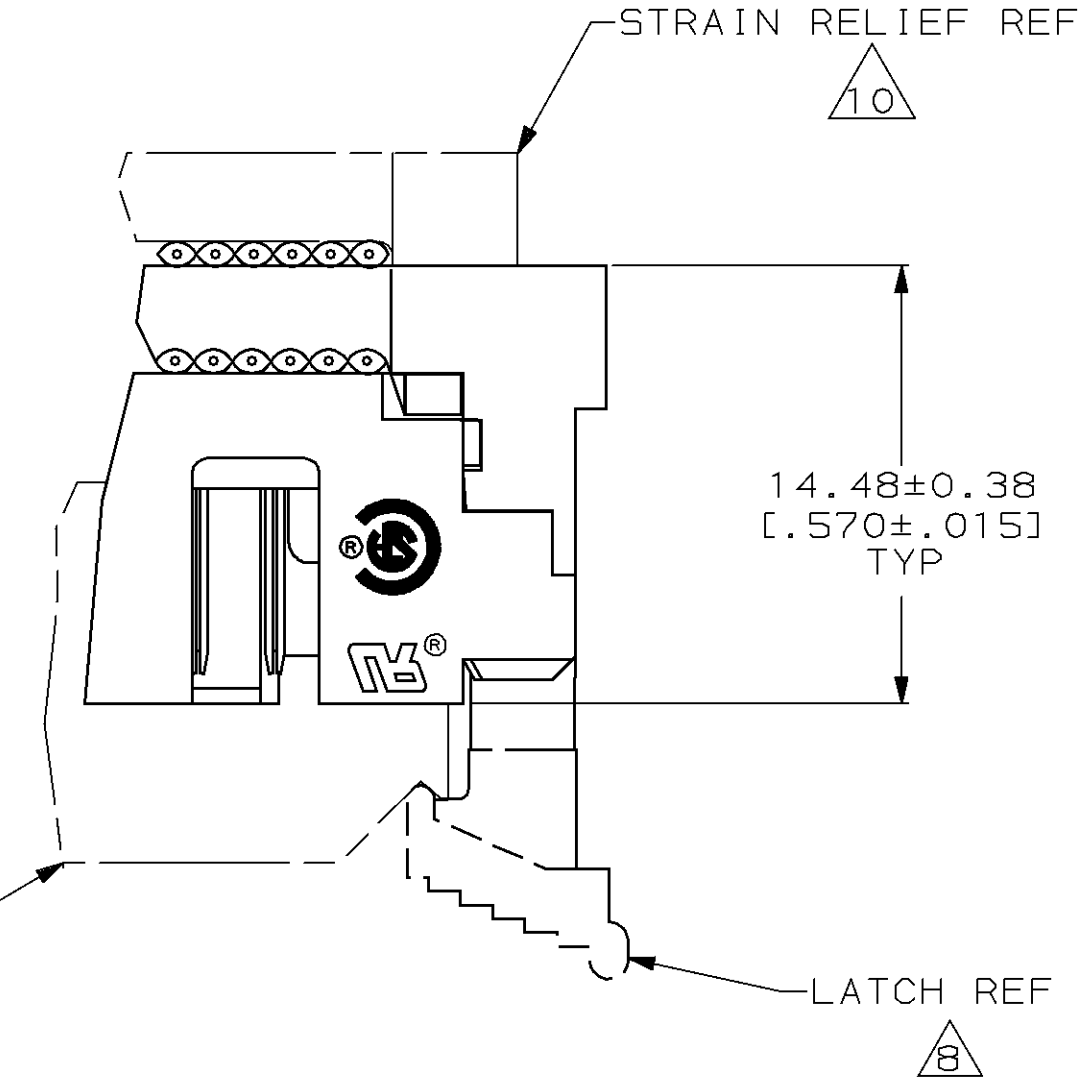
TERMINATED ASSEMBLY (ASSEMBLED BY CUSTOMER)
