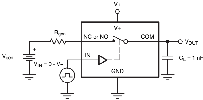
Figure 3. Charge Injection
