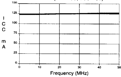
SUPPLY CURRENT vs. INPUT FREQUENCY ATV750B (TA = 25C, VCC = 5V)
