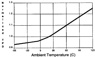
NORMALIZED TPD vs. TEMPERATURE
