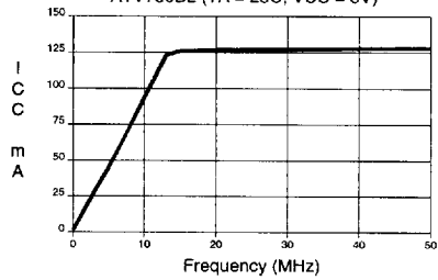
SUPPLY CURRENT vs. INPUT FREQUENCY ATV750BL (TA = 25C, VCC = 5V)
