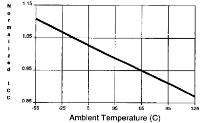
NORMALIZED ICC vs. AMBIENT TEMP. f = 50 MHz
