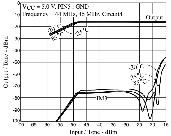
Intermodulation Characteristic
