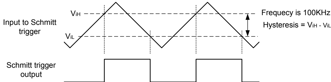
Figure 15. Schmitt Trigger Timing Diagram
