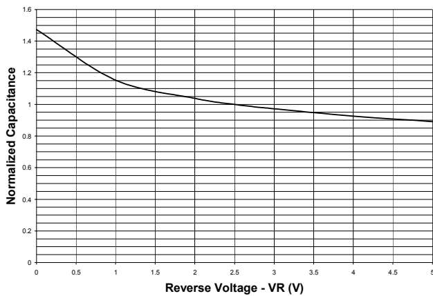
Capacitance vs. Reverse Voltage (Normalized to 2.5 volts)
