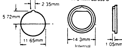
PANEL CUTOUT
