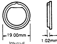
Internal Dimension 12.70mm DIA. 11.94mm across D
