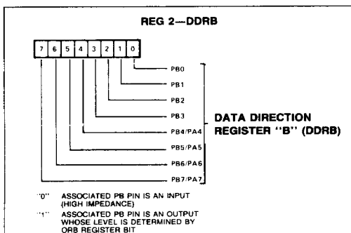
Figure 7. Data Direction Register B (DORB)
