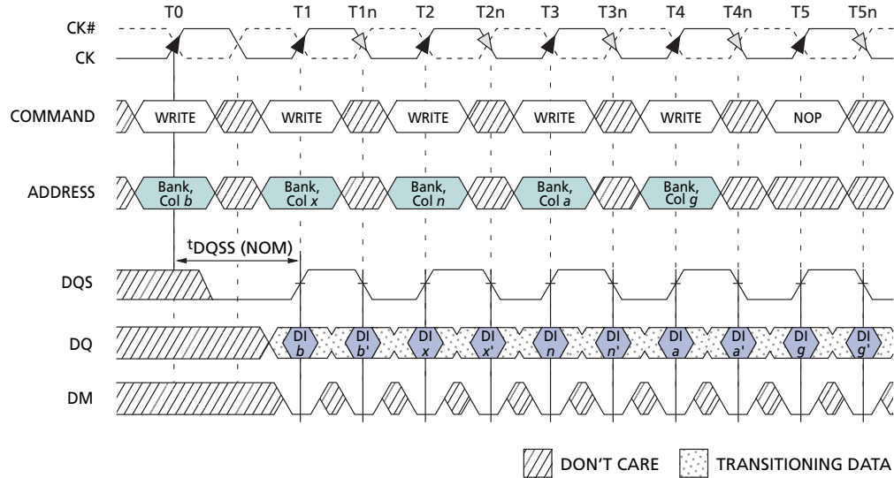
Figure 22: Random WRITE Cycles
