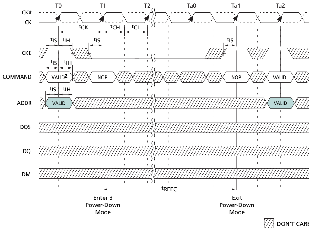
Figure 44: Power-Down Mode
