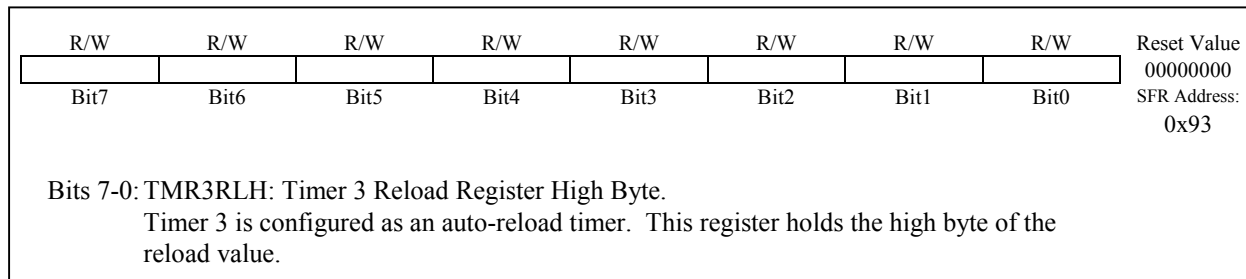
Figure 17.22. TMR3RLH: Timer 3 Reload Register High Byte
