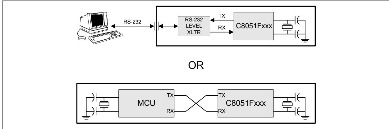
Figure 16.5. UART Modes 1, 2, and 3 Interconnect Diagram
