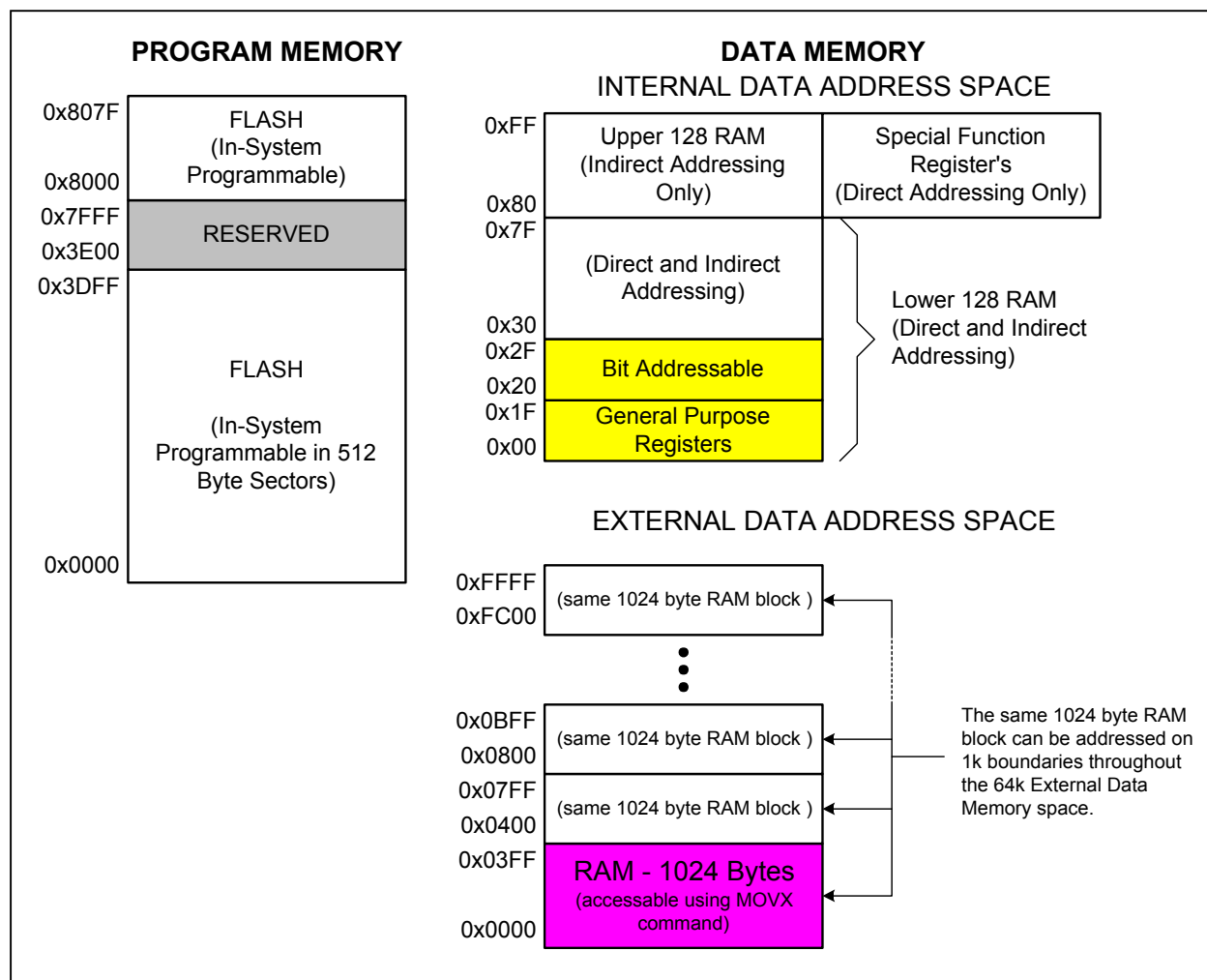
Figure 8.2. Memory Map
