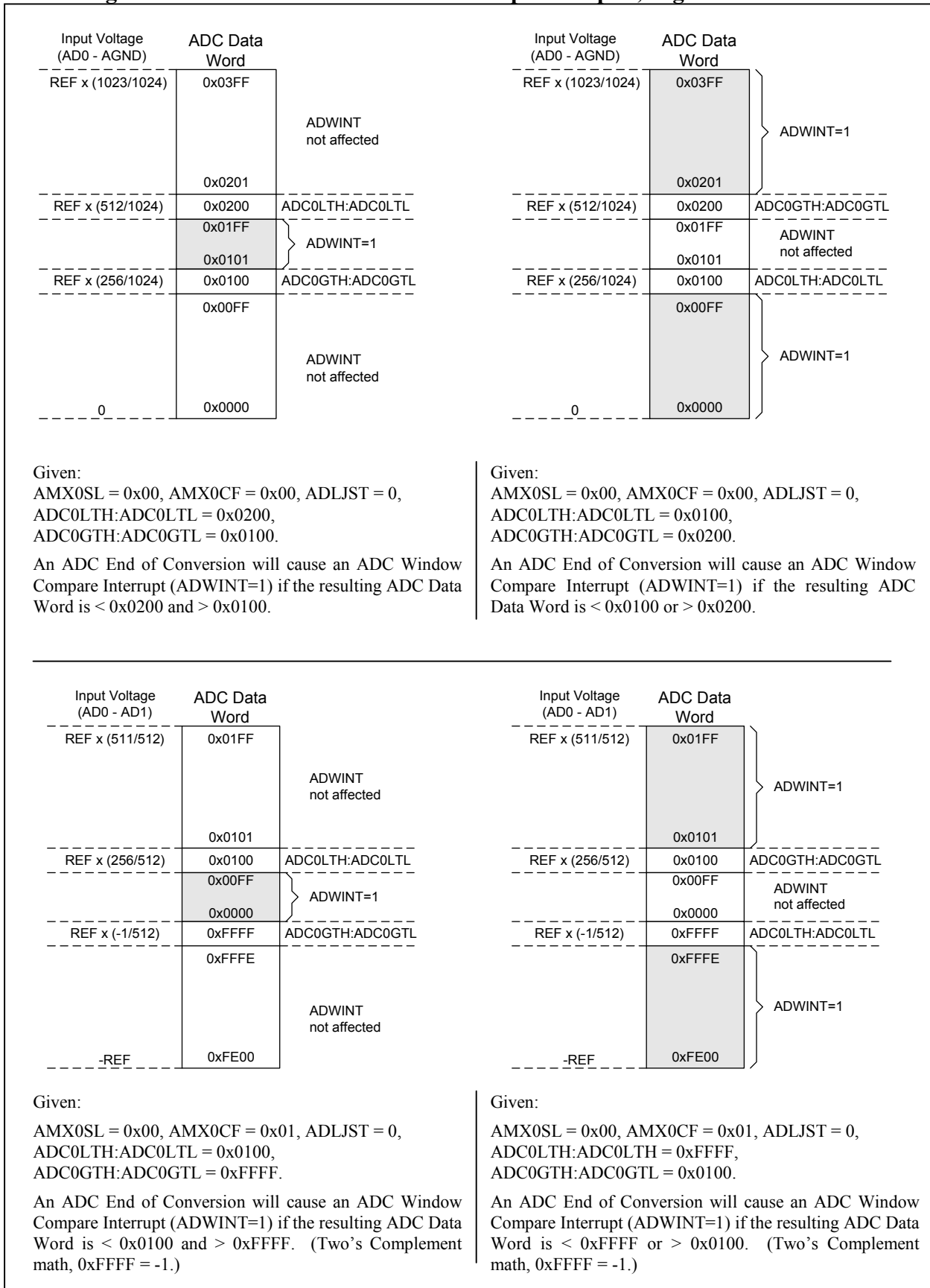
Figure 5.14. 10-Bit ADC Window Interrupt Examples, Right Justified Data
