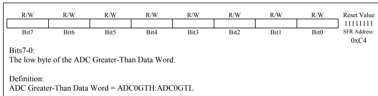
Figure 5.11. ADC0GTL: ADC Greater-Than Data Low Byte Register
