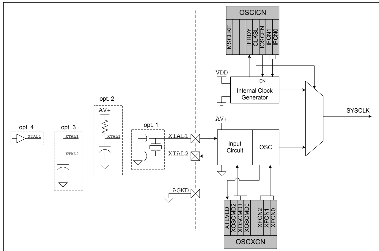
Figure 12.1. Oscillator Diagram
