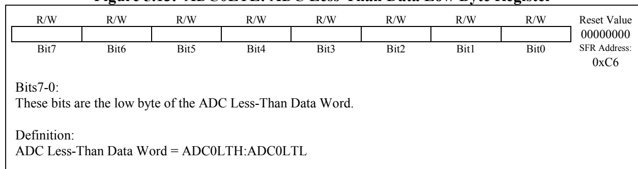
Figure 5.13. ADC0LTL: ADC Less-Than Data Low Byte Register
