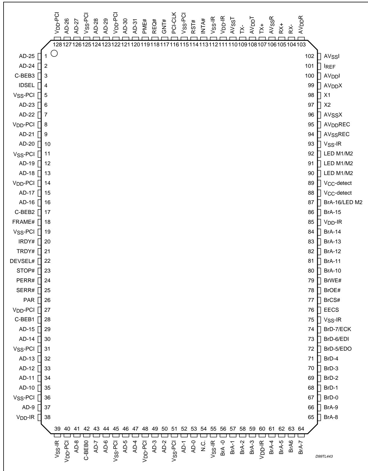
Figure 3. Pin Connection
