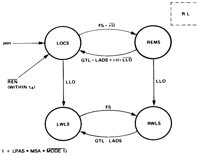
Figure A-1. 8291A State Diagrams (Continued)
