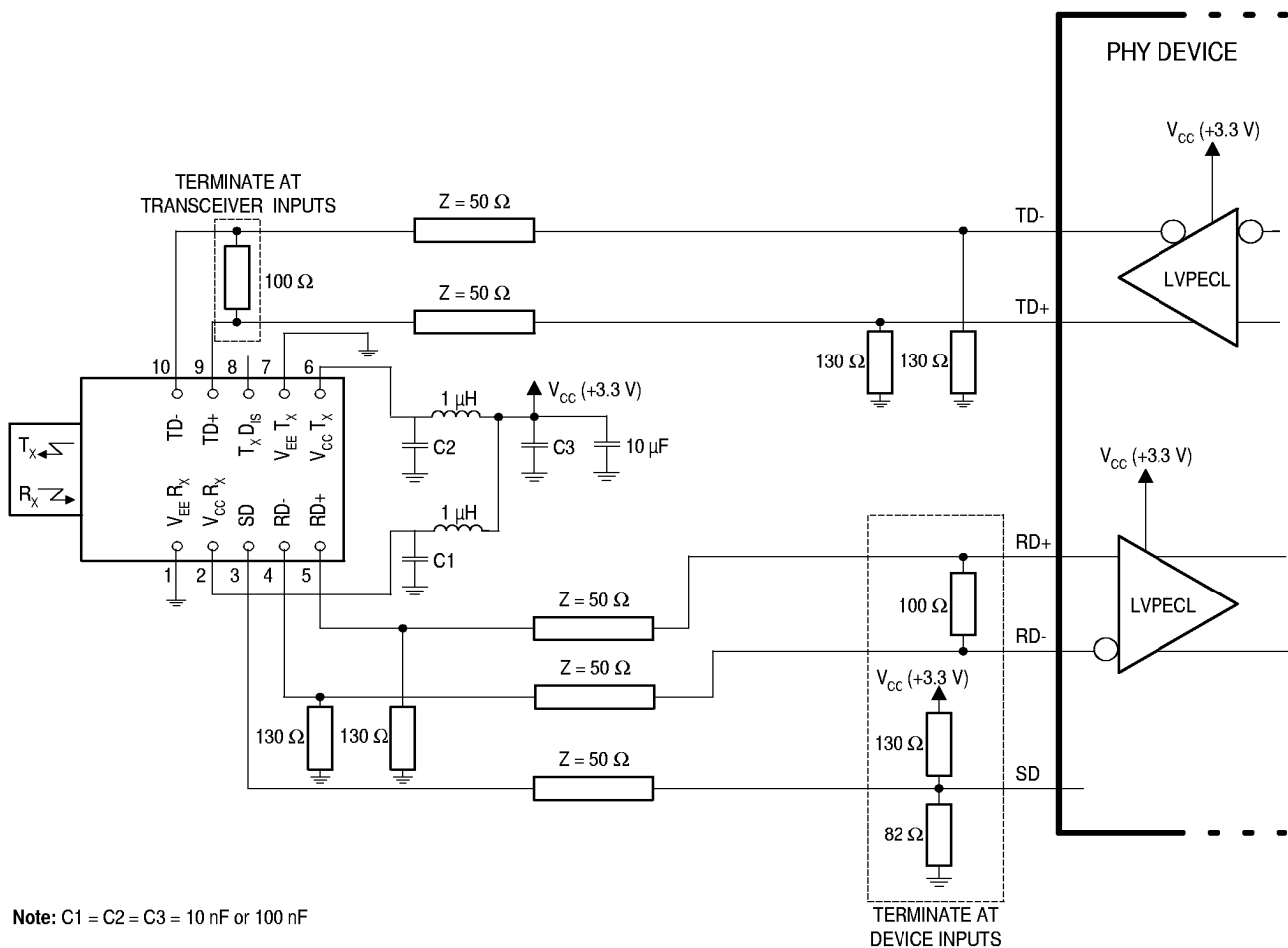
Figure 3. +3.3 V Transceiver Interface with +3.3 V LVPECL Device
