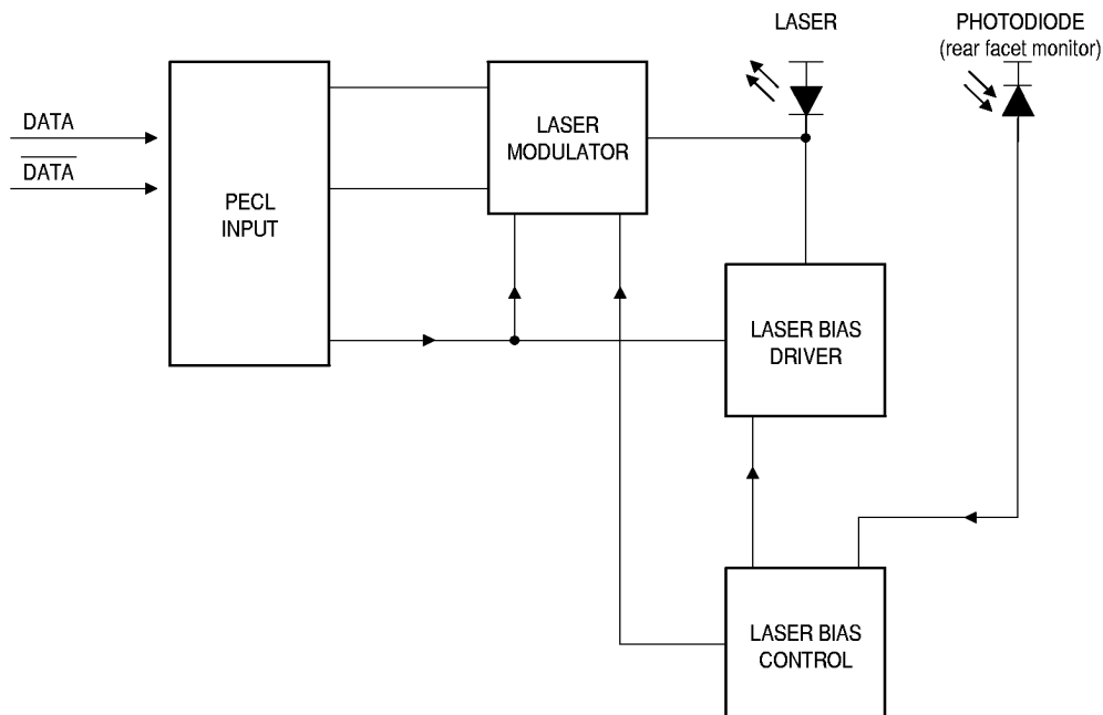
Figure 2. Simplified Transmitter Schematic
