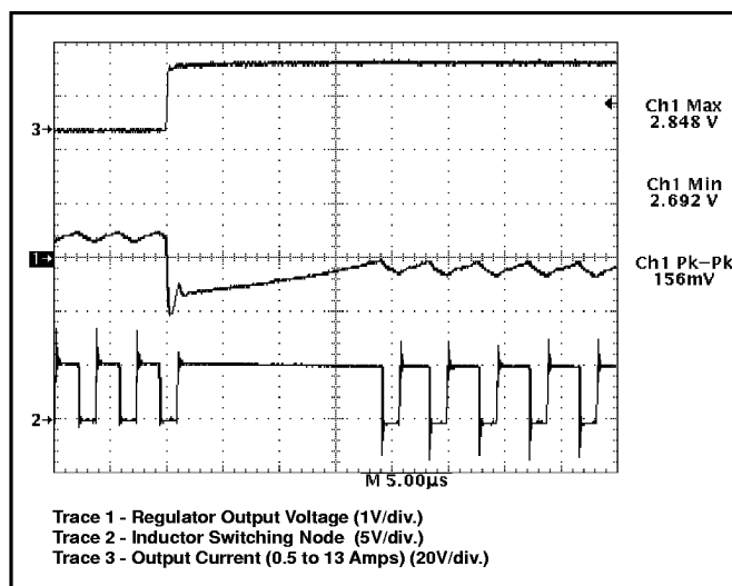
Figure 8: CS-5151H demonstration board response to 13A load turn on (output set for 2.8V). Upon completing a normal off time, the V^{2T} control loop immediately connects the inductor to the input voltage, providing 100% duty cycle. Regulation is achieved in less than 20µs.
