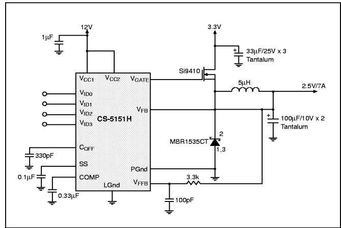
Figure 21: 3.3V to 2.5V/7A converter with 12V bias.
