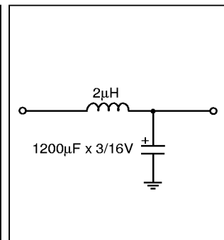
Figure 17: Input Filter
