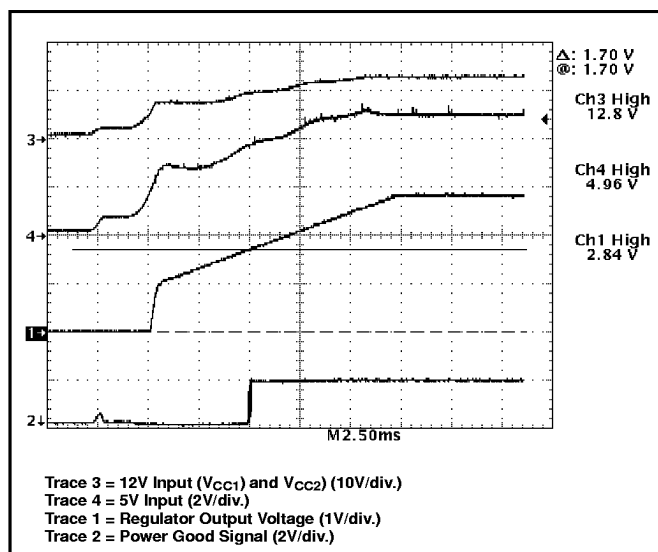
Figure 14: CS-5151H demonstration board during power up. Power Good signal is activated when output voltage reaches 1.70V.
