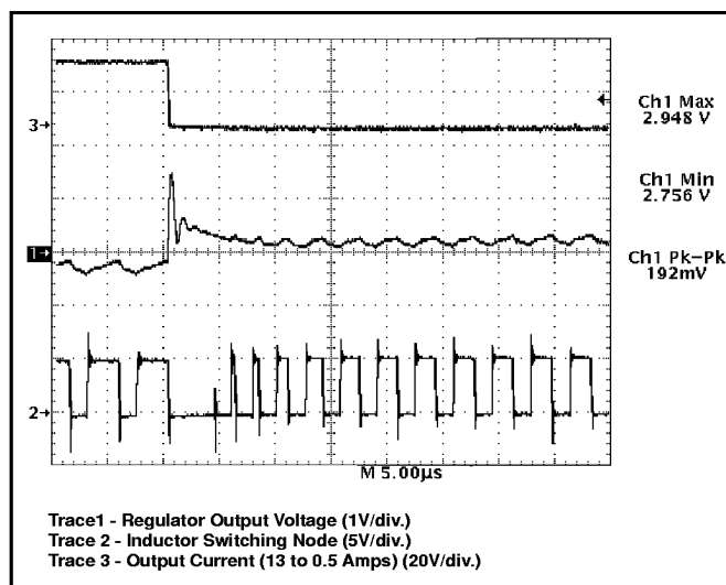
Figure 9: CS-5151H demonstration board response to 13A load turn off (output set for 2.8V). V^{2T} control topology immediately connects inductor to ground, providing 0% duty cycle. Regulation is achieved in less than 10µs.
