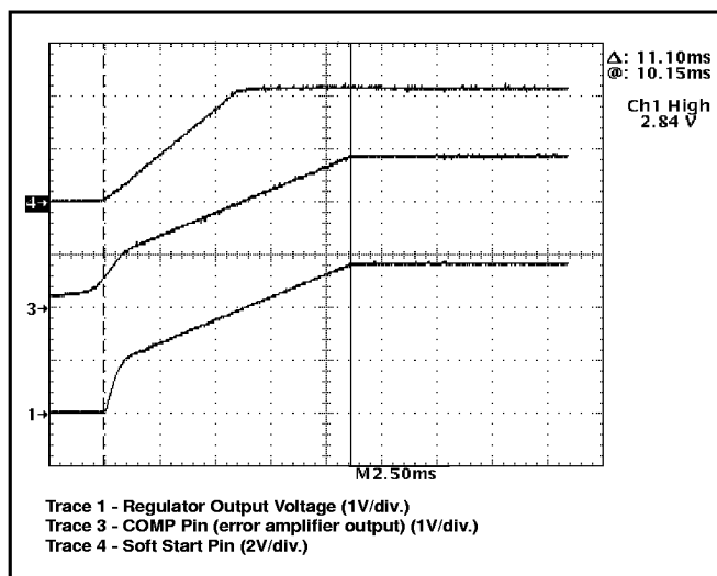
Figure 3: CS-5151H demonstration board startup waveforms.
