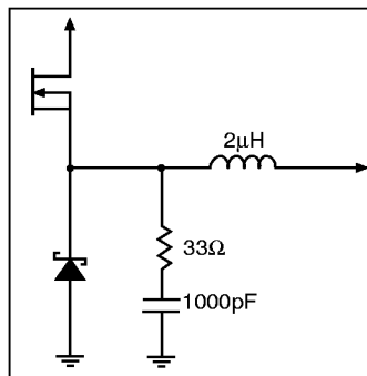
Figure 16: Filter components
