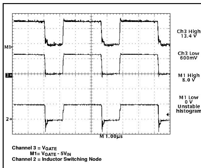
Figure 15: CS-5151H gate drive waveforms depicting rail to rail swing.
