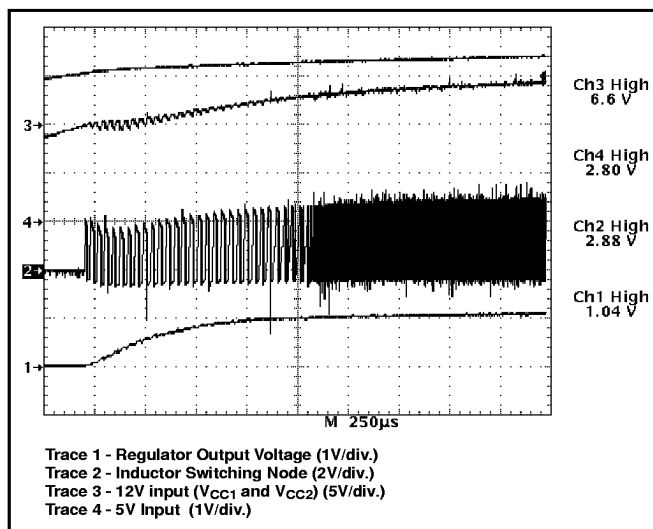
Figure 2: CS-5151H demonstration board startup in response to increasing 12V and 5V input voltages. Extended off time is followed by normal off time operation when output voltage achieves regulation to the error amplifier output.
