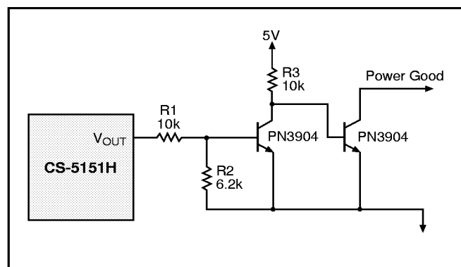
Figure 13: Implementing Power Good with the CS-5151H.
