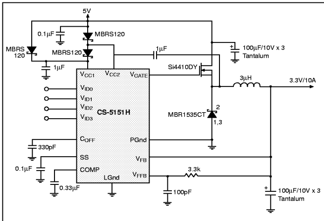
Figure 19: 5V to 3.3V/10A converter.
