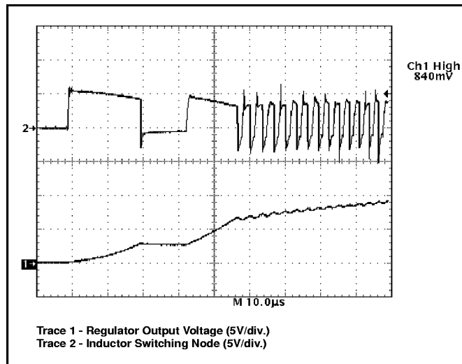
Figure 4: CS-5151H demonstration board enable startup waveforms.
