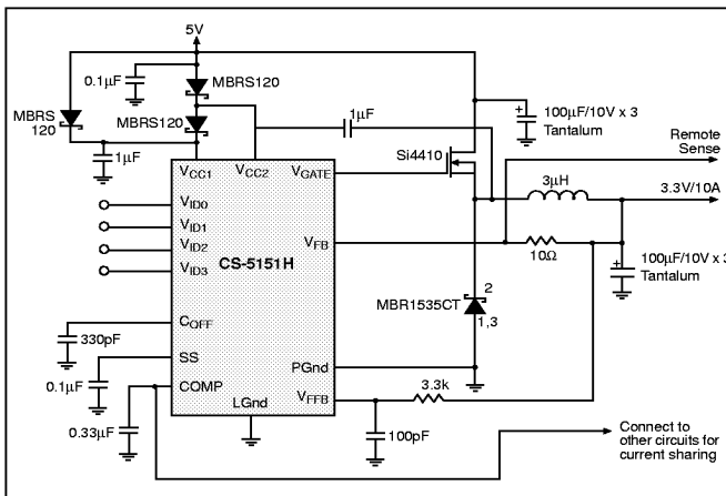
Figure 20: 5V to 3.3V/10A converter with current sharing.
