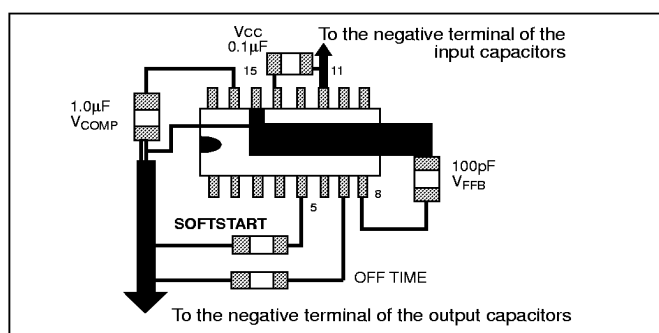
Figure 18: Layout Guidelines
