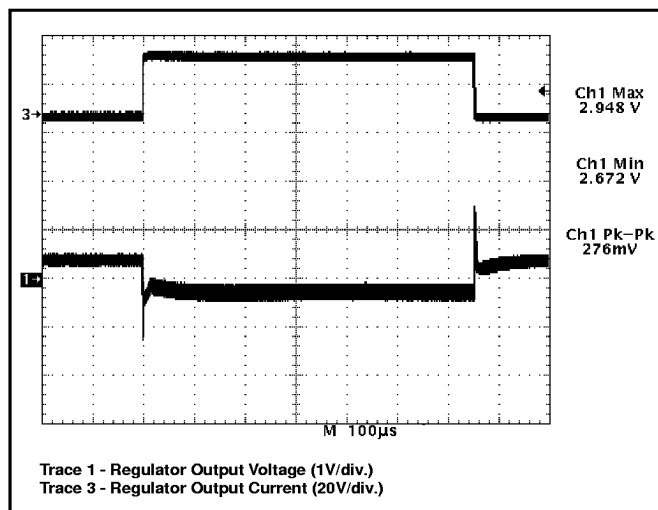
Figure 7: CS-5151H demonstration board response to a 0.5 to 13A load pulse (output set for 2.8V).
