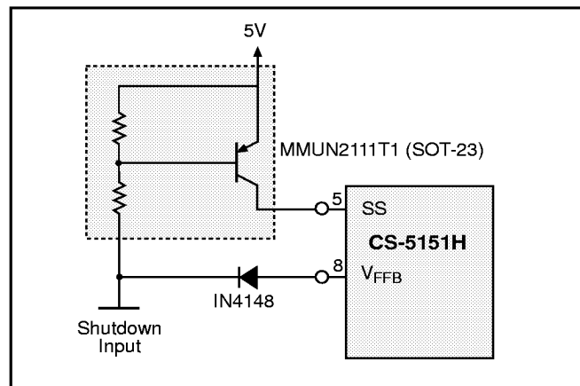
Figure 12: Implementing shutdown with the CS-5151H.
